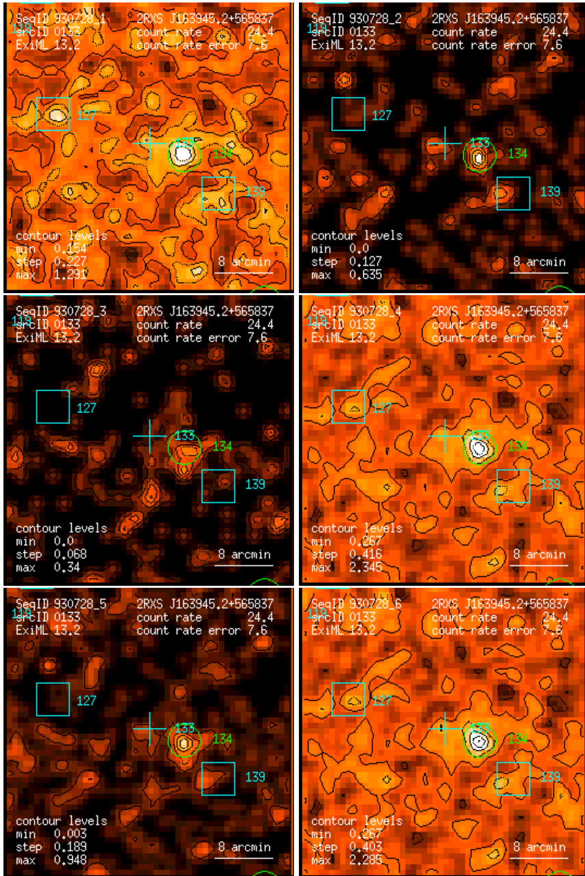
Figure 133: RASS 930728: detection 0133: band rate images, Gaussian filter: (1) PSPC channels 11 – 41, (2) 52 – 90, (3) 91 – 201, (4) 11 – 235, (5) 52 – 201, (6) 11 – 201. Broad band rates in counts/ks. Band rate contour levels in counts/ks/arcmin 2 .
