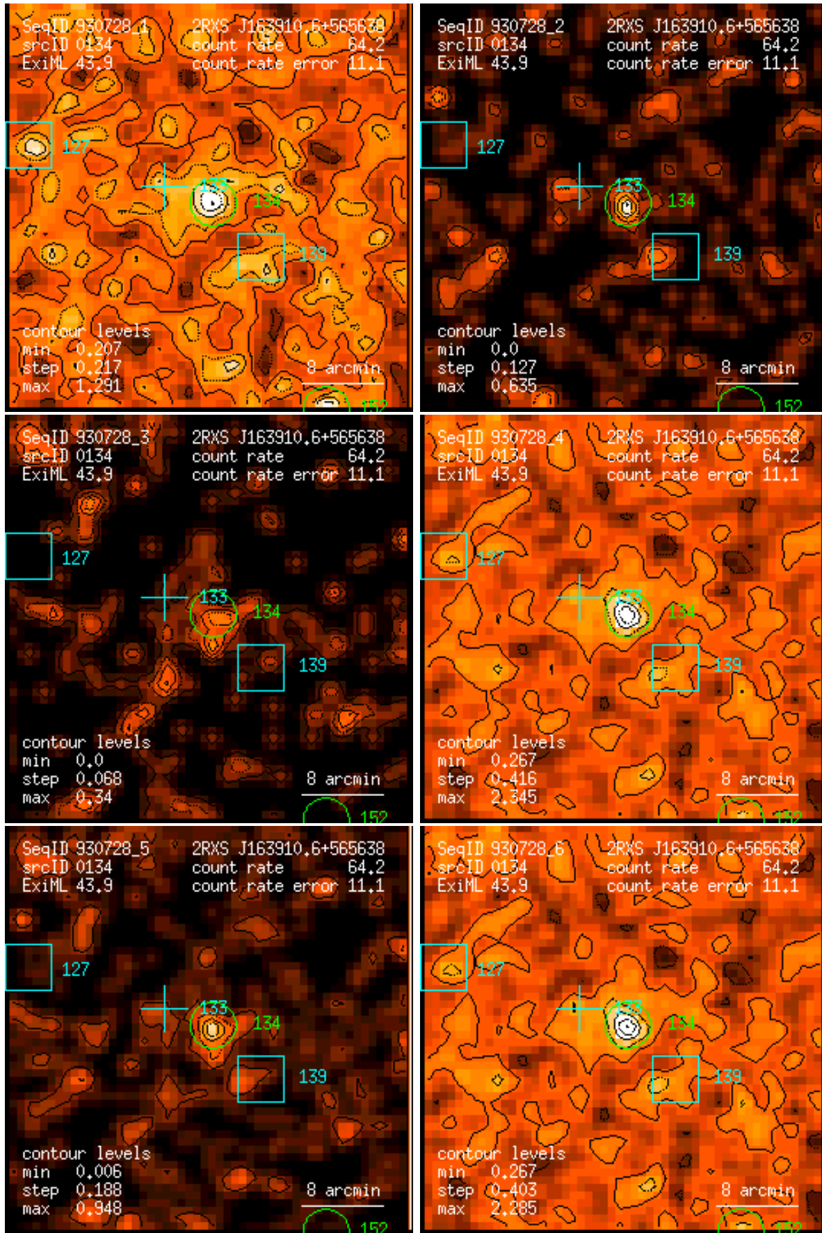
Figure 134: RASS 930728: detection 0134: band rate images, Gaussian filter: (1) PSPC channels 11 – 41, (2) 52 – 90, (3) 91 – 201, (4) 11 – 235, (5) 52 – 201, (6) 11 – 201. Broad band rates in counts/ks. Band rate contour levels in counts/ks/arcmin 2 .
