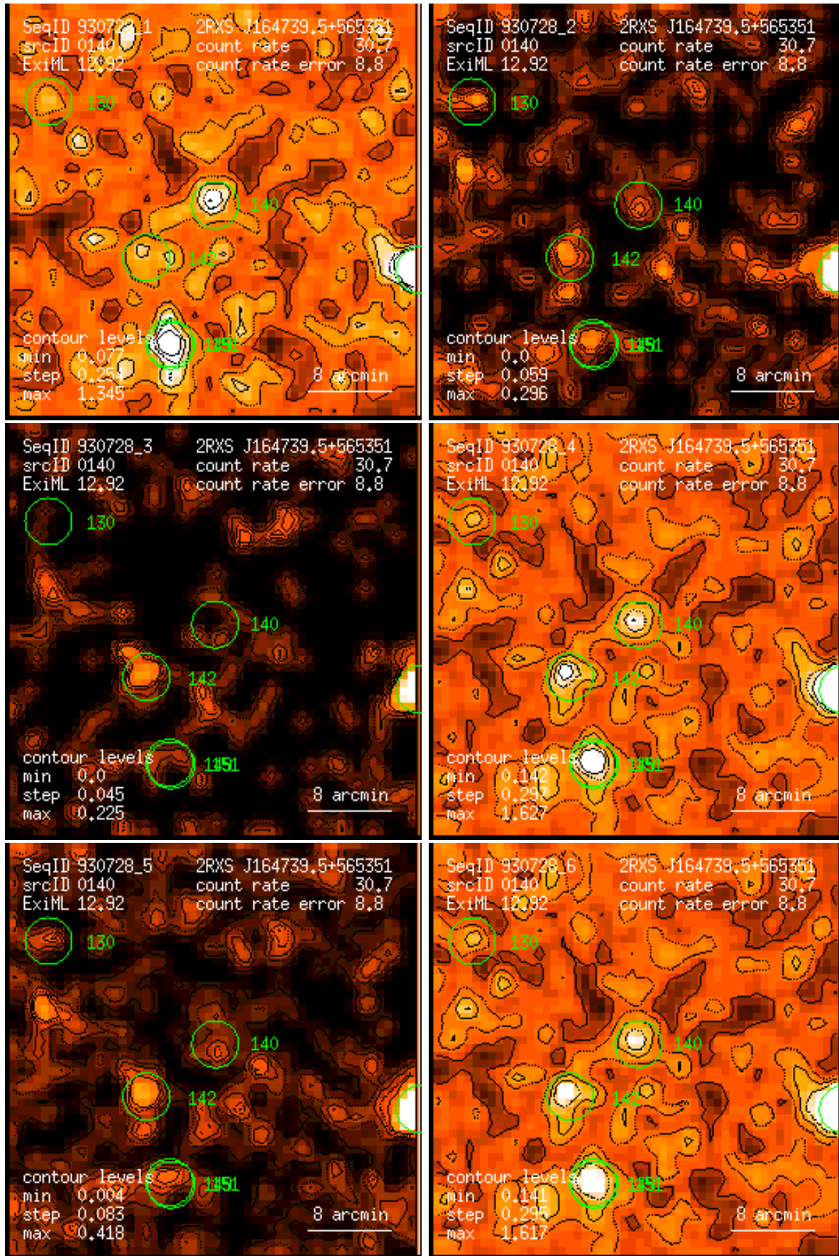
Figure 140: RASS 930728: detection 0140: band rate images, Gaussian filter: (1) PSPC channels 11 – 41, (2) 52 – 90, (3) 91 – 201, (4) 11 – 235, (5) 52 – 201, (6) 11 – 201. Broad band rates in counts/ks. Band rate contour levels in counts/ks/arcmin 2 .
