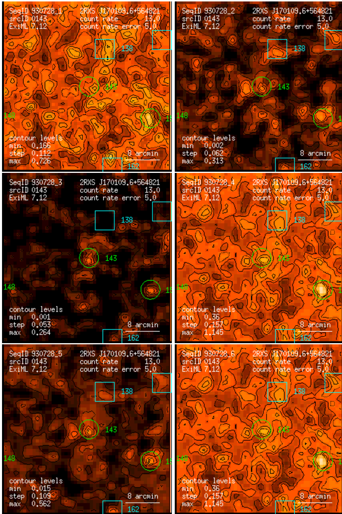
Figure 143: RASS 930728: detection 0143: band rate images, Gaussian filter: (1) PSPC channels 11 – 41, (2) 52 – 90, (3) 91 – 201, (4) 11 – 235, (5) 52 – 201, (6) 11 – 201. Broad band rates in counts/ks. Band rate contour levels in counts/ks/arcmin 2 .
