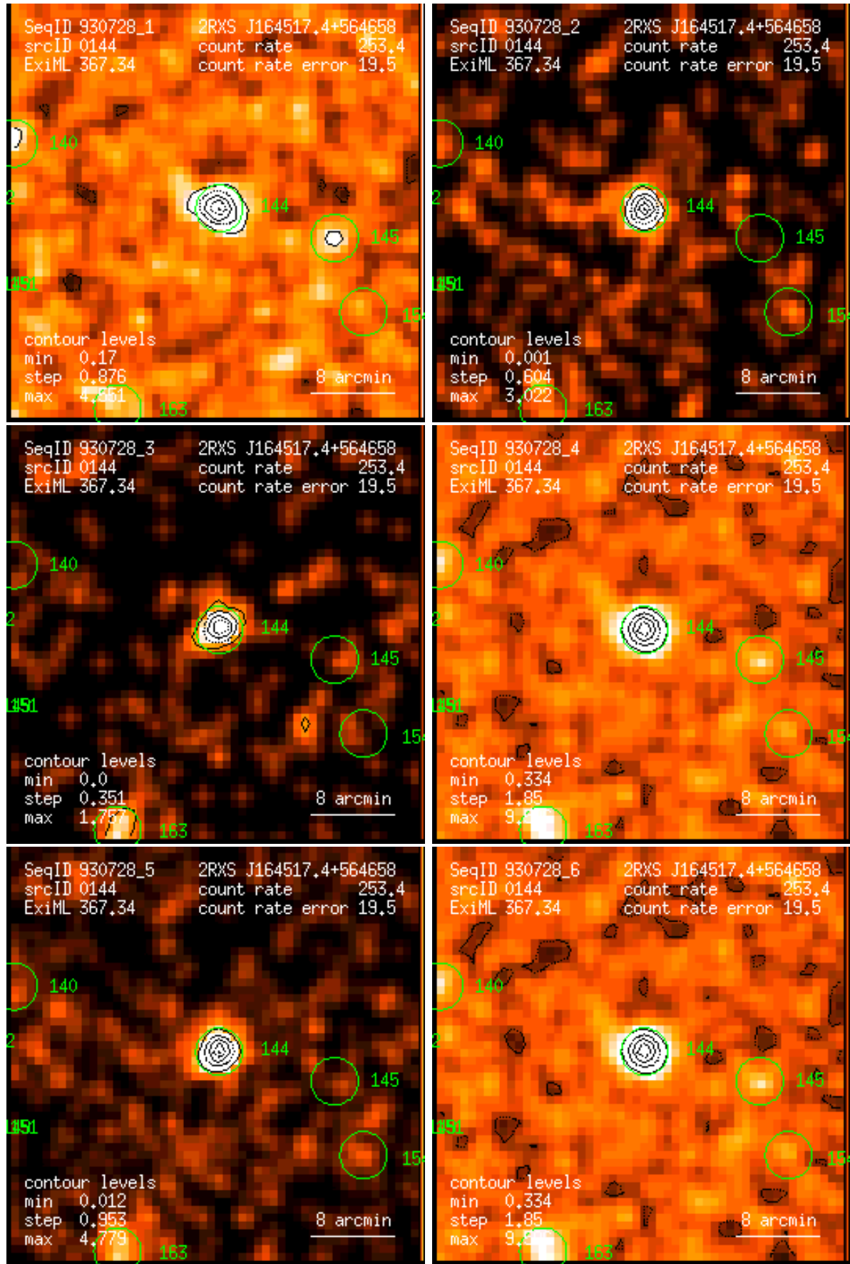
Figure 144: RASS 930728: detection 0144: band rate images, Gaussian filter: (1) PSPC channels 11 – 41, (2) 52 – 90, (3) 91 – 201, (4) 11 – 235, (5) 52 – 201, (6) 11 – 201. Broad band rates in counts/ks. Band rate contour levels in counts/ks/arcmin 2 .
