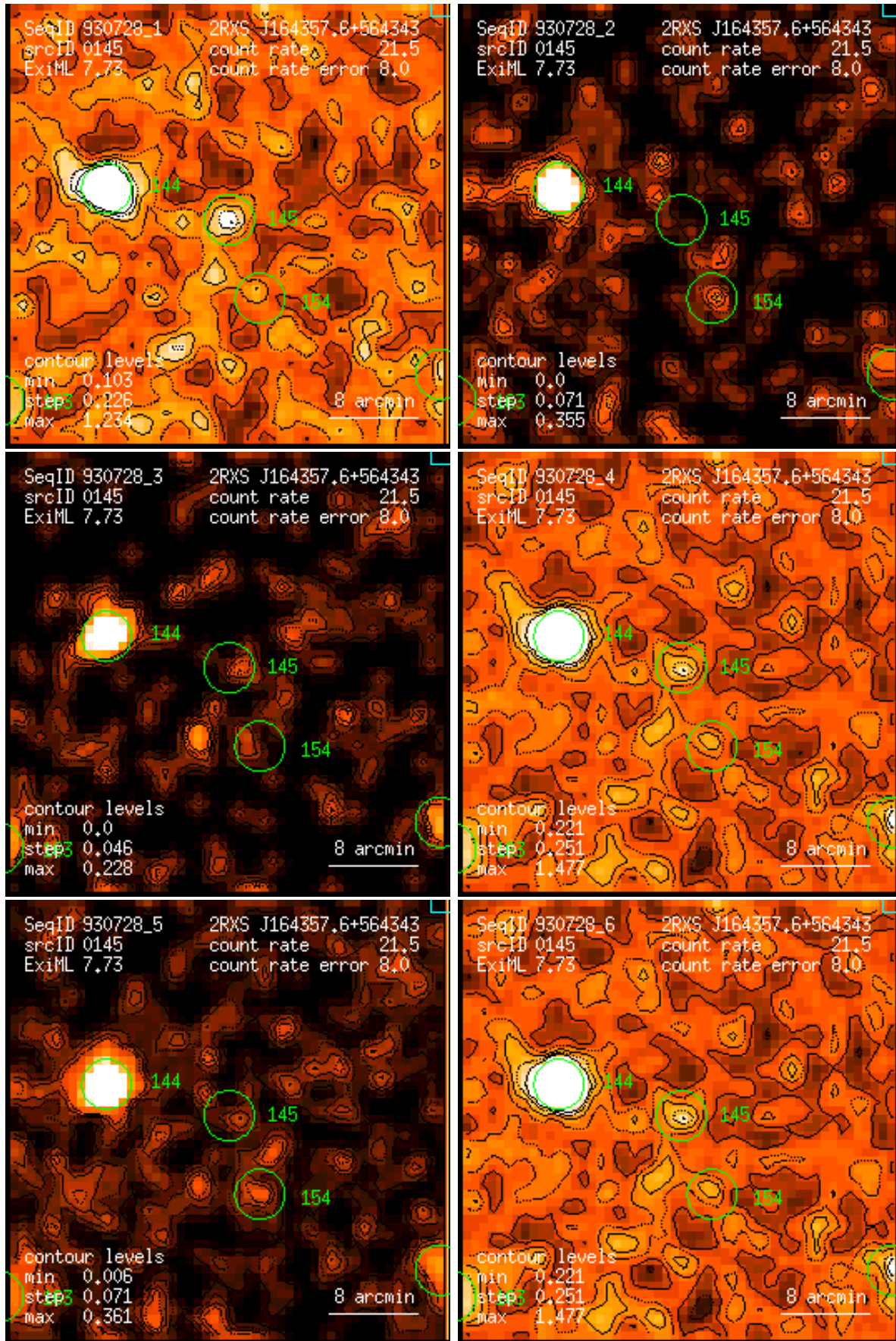
Figure 145: RASS 930728: detection 0145: band rate images, Gaussian filter: (1) PSPC channels 11 – 41, (2) 52 – 90, (3) 91 – 201, (4) 11 – 235, (5) 52 – 201, (6) 11 – 201. Broad band rates in counts/ks. Band rate contour levels in counts/ks/arcmin 2 .
