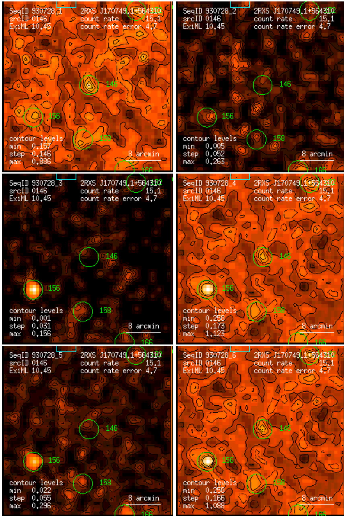
Figure 146: RASS 930728: detection 0146: band rate images, Gaussian filter: (1) PSPC channels 11 – 41, (2) 52 – 90, (3) 91 – 201, (4) 11 – 235, (5) 52 – 201, (6) 11 – 201. Broad band rates in counts/ks. Band rate contour levels in counts/ks/arcmin 2 .
