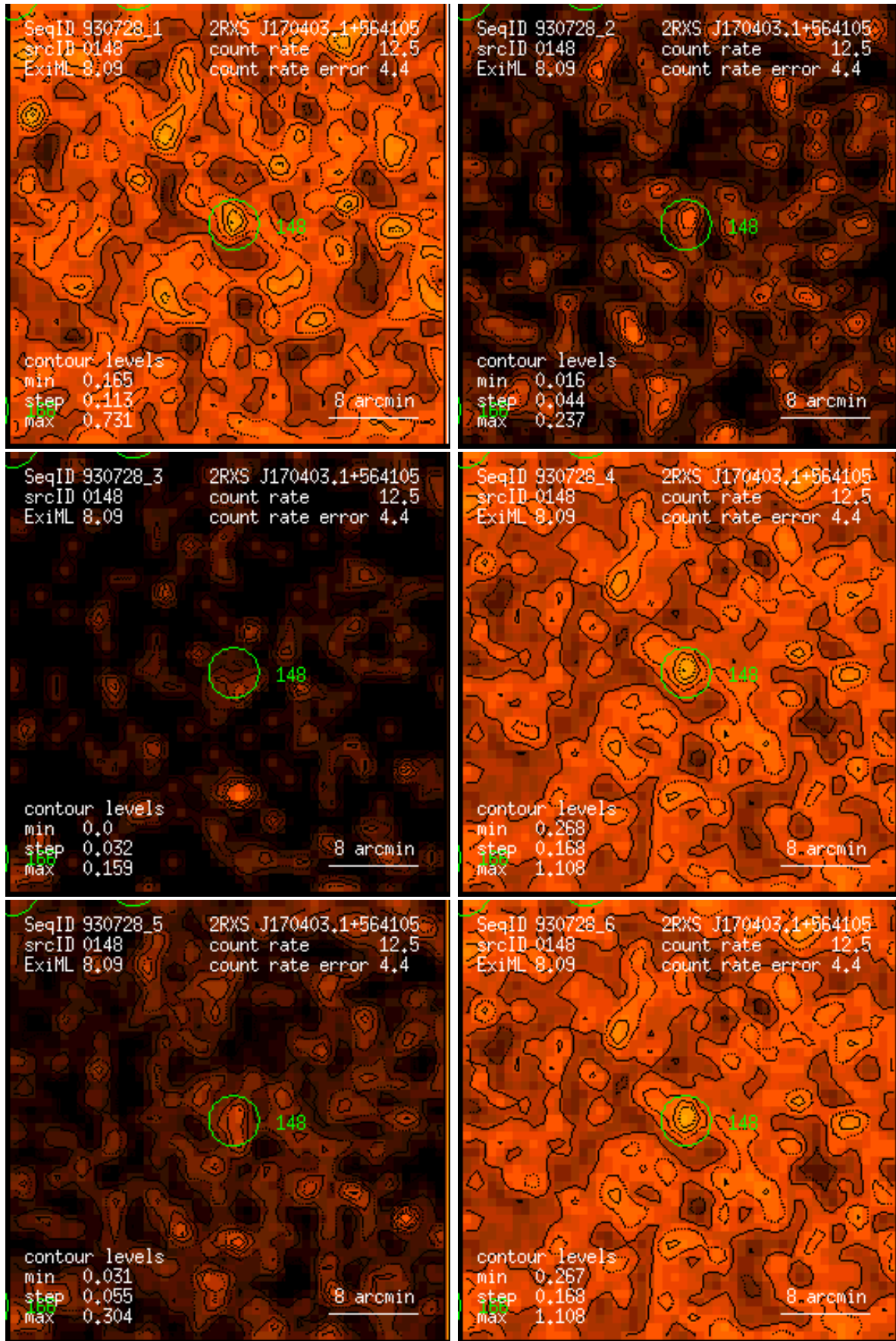
Figure 148: RASS 930728: detection 0148: band rate images, Gaussian filter: (1) PSPC channels 11 – 41, (2) 52 – 90, (3) 91 – 201, (4) 11 – 235, (5) 52 – 201, (6) 11 – 201. Broad band rates in counts/ks. Band rate contour levels in counts/ks/arcmin 2 .
