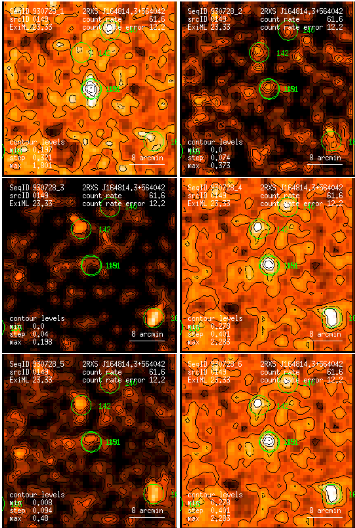
Figure 149: RASS 930728: detection 0149: band rate images, Gaussian filter: (1) PSPC channels 11 – 41, (2) 52 – 90, (3) 91 – 201, (4) 11 – 235, (5) 52 – 201, (6) 11 – 201. Broad band rates in counts/ks. Band rate contour levels in counts/ks/arcmin 2 .
