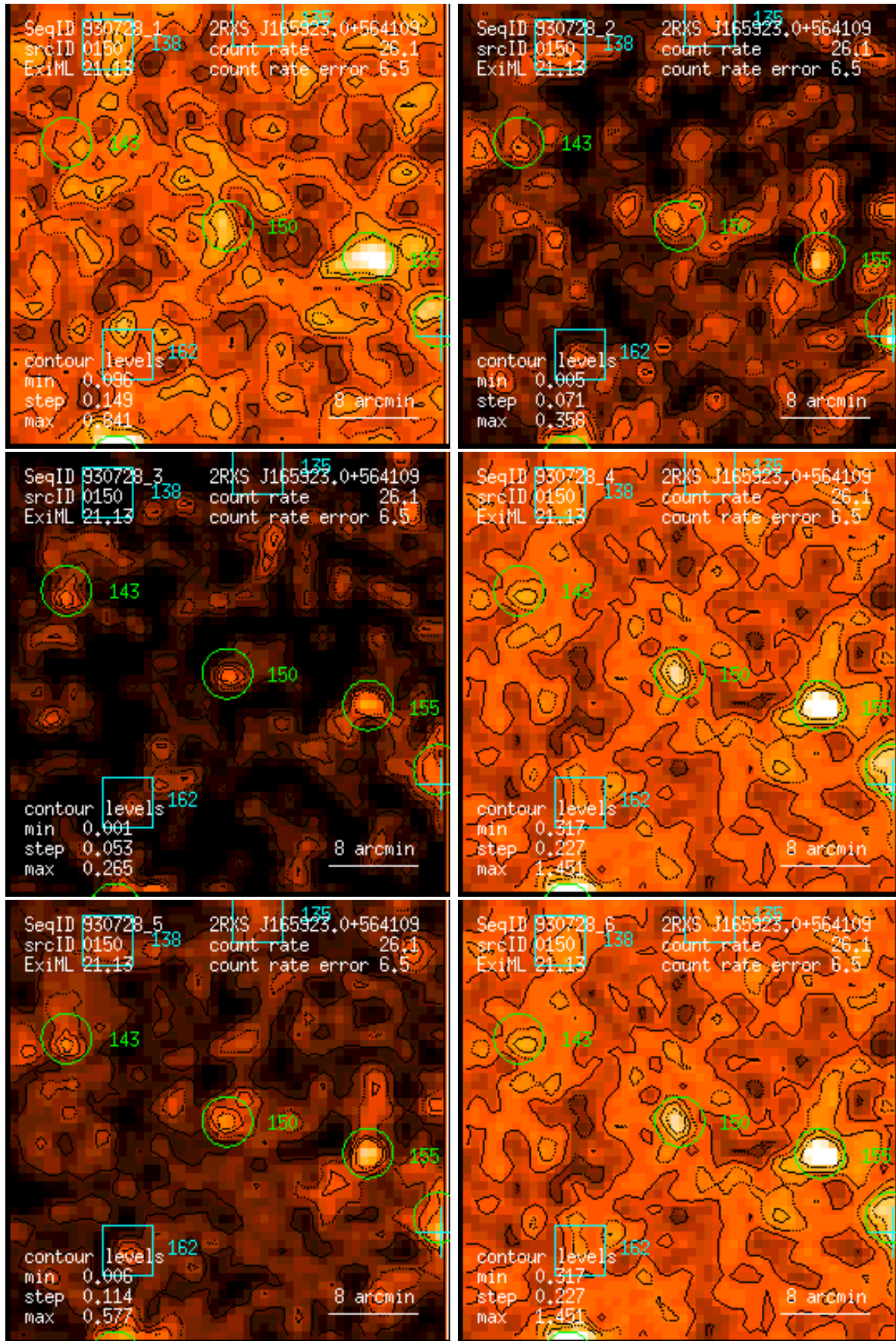
Figure 150: RASS 930728: detection 0150: band rate images, Gaussian filter: (1) PSPC channels 11 – 41, (2) 52 – 90, (3) 91 – 201, (4) 11 – 235, (5) 52 – 201, (6) 11 – 201. Broad band rates in counts/ks. Band rate contour levels in counts/ks/arcmin 2 .
