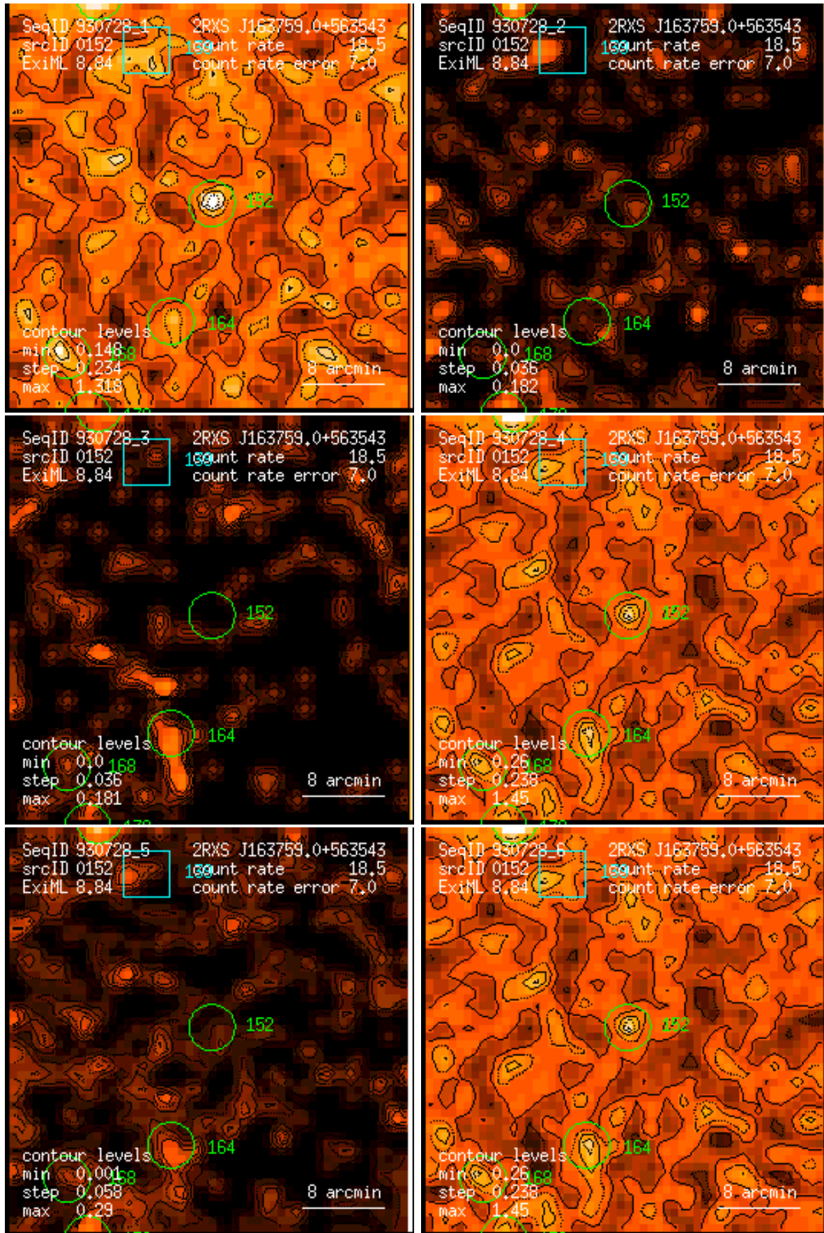
Figure 152: RASS 930728: detection 0152: band rate images, Gaussian filter: (1) PSPC channels 11 – 41, (2) 52 – 90, (3) 91 – 201, (4) 11 – 235, (5) 52 – 201, (6) 11 – 201. Broad band rates in counts/ks. Band rate contour levels in counts/ks/arcmin 2 .
