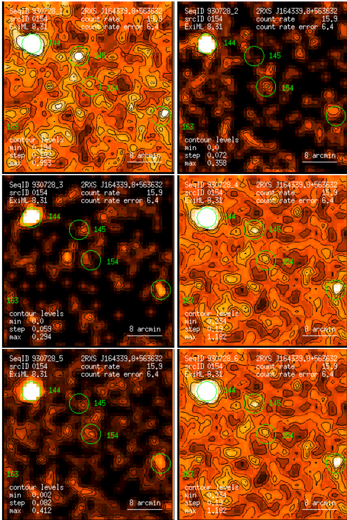
Figure 154: RASS 930728: detection 0154: band rate images, Gaussian filter: (1) PSPC channels 11 – 41, (2) 52 – 90, (3) 91 – 201, (4) 11 – 235, (5) 52 – 201, (6) 11 – 201. Broad band rates in counts/ks. Band rate contour levels in counts/ks/arcmin 2 .
