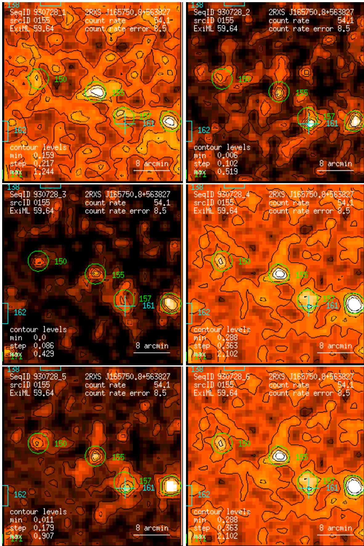
Figure 155: RASS 930728: detection 0155: band rate images, Gaussian filter: (1) PSPC channels 11 – 41, (2) 52 – 90, (3) 91 – 201, (4) 11 – 235, (5) 52 – 201, (6) 11 – 201. Broad band rates in counts/ks. Band rate contour levels in counts/ks/arcmin 2 .
