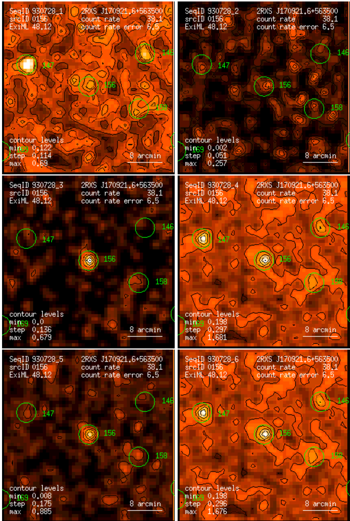
Figure 156: RASS 930728: detection 0156: band rate images, Gaussian filter: (1) PSPC channels 11 – 41, (2) 52 – 90, (3) 91 – 201, (4) 11 – 235, (5) 52 – 201, (6) 11 – 201. Broad band rates in counts/ks. Band rate contour levels in counts/ks/arcmin 2 .
