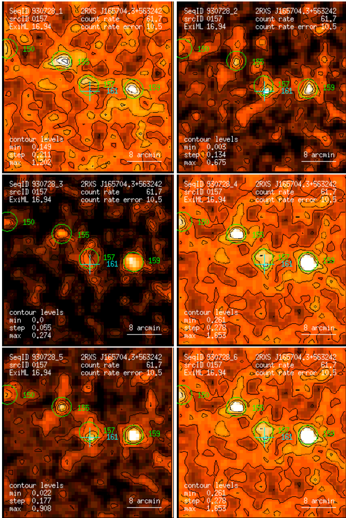
Figure 157: RASS 930728: detection 0157: band rate images, Gaussian filter: (1) PSPC channels 11 – 41, (2) 52 – 90, (3) 91 – 201, (4) 11 – 235, (5) 52 – 201, (6) 11 – 201. Broad band rates in counts/ks. Band rate contour levels in counts/ks/arcmin 2 .
