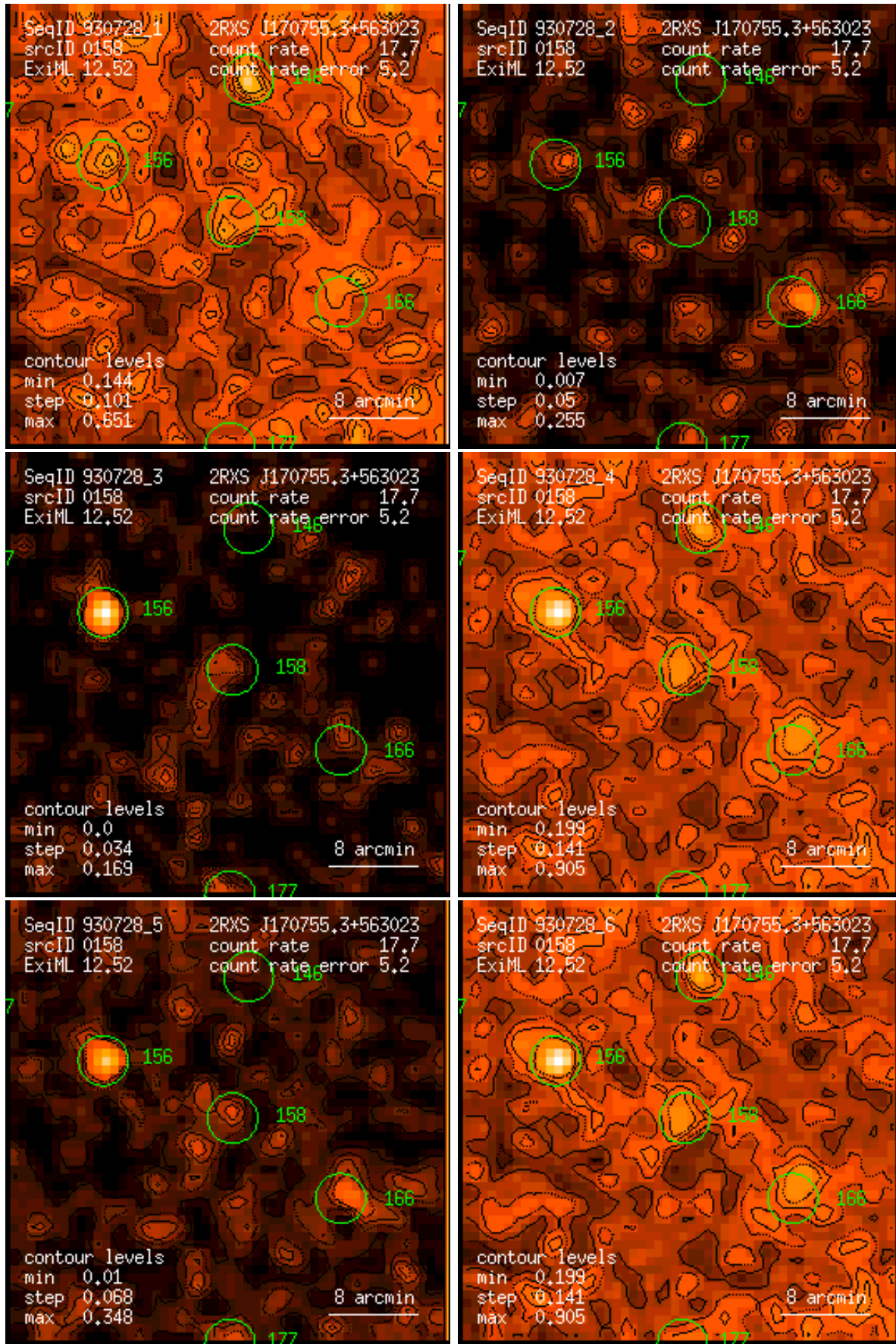
Figure 158: RASS 930728: detection 0158: band rate images, Gaussian filter: (1) PSPC channels 11 – 41, (2) 52 – 90, (3) 91 – 201, (4) 11 – 235, (5) 52 – 201, (6) 11 – 201. Broad band rates in counts/ks. Band rate contour levels in counts/ks/arcmin 2 .
