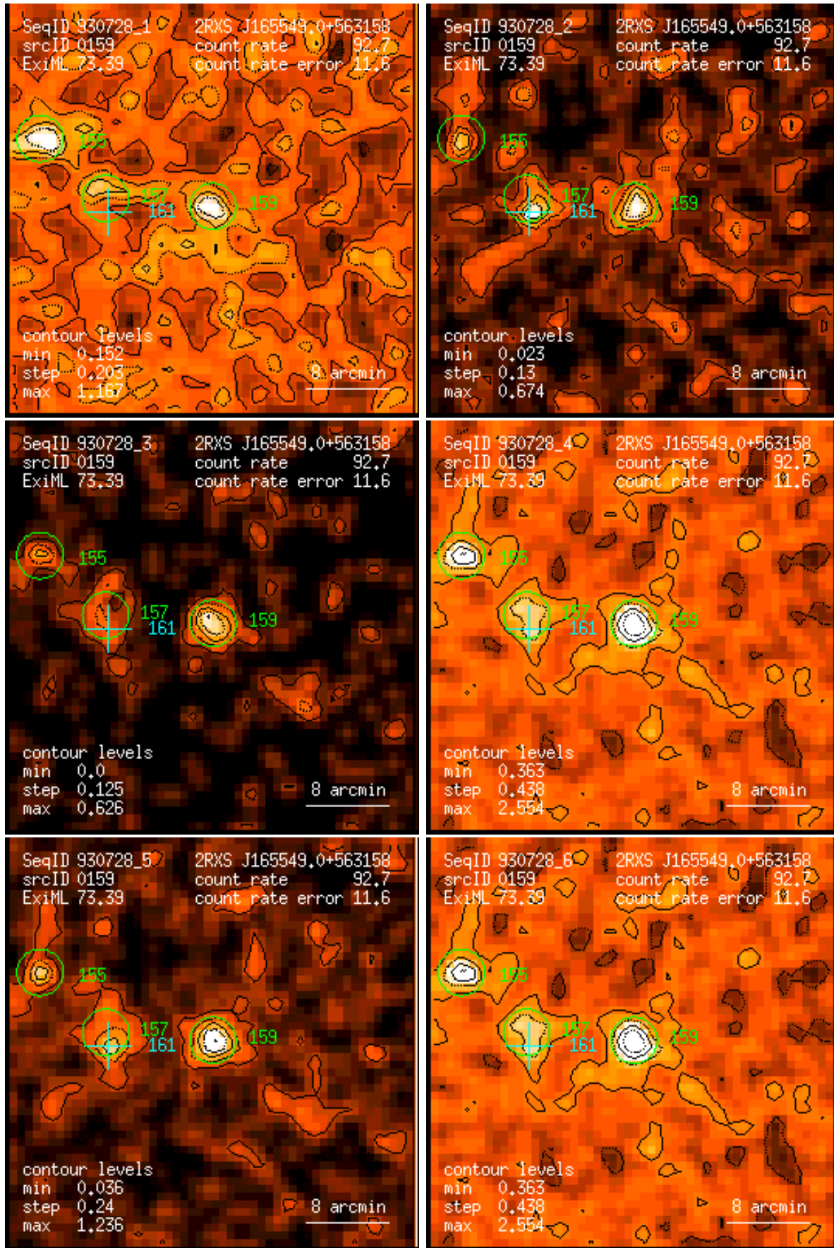
Figure 159: RASS 930728: detection 0159: band rate images, Gaussian filter: (1) PSPC channels 11 – 41, (2) 52 – 90, (3) 91 – 201, (4) 11 – 235, (5) 52 – 201, (6) 11 – 201. Broad band rates in counts/ks. Band rate contour levels in counts/ks/arcmin 2 .
