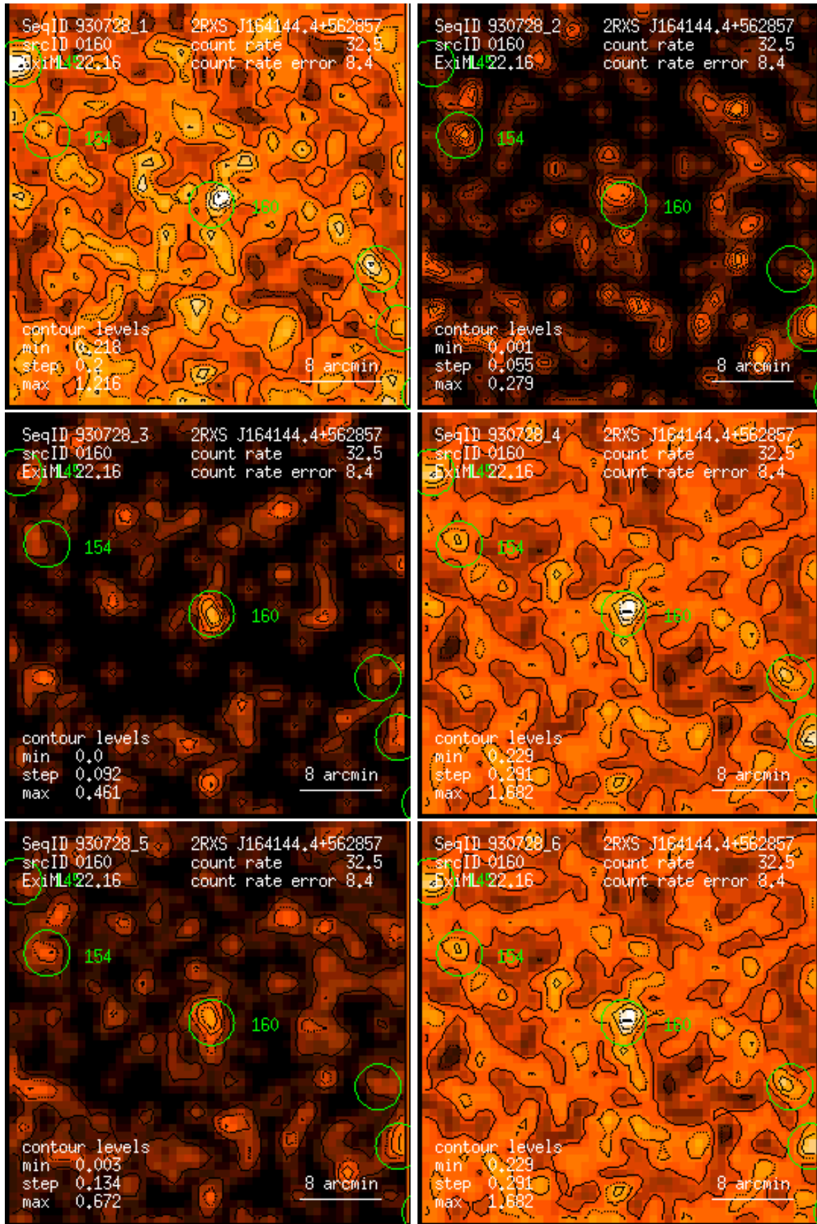
Figure 160: RASS 930728: detection 0160: band rate images, Gaussian filter: (1) PSPC channels 11 – 41, (2) 52 – 90, (3) 91 – 201, (4) 11 – 235, (5) 52 – 201, (6) 11 – 201. Broad band rates in counts/ks. Band rate contour levels in counts/ks/arcmin 2 .
