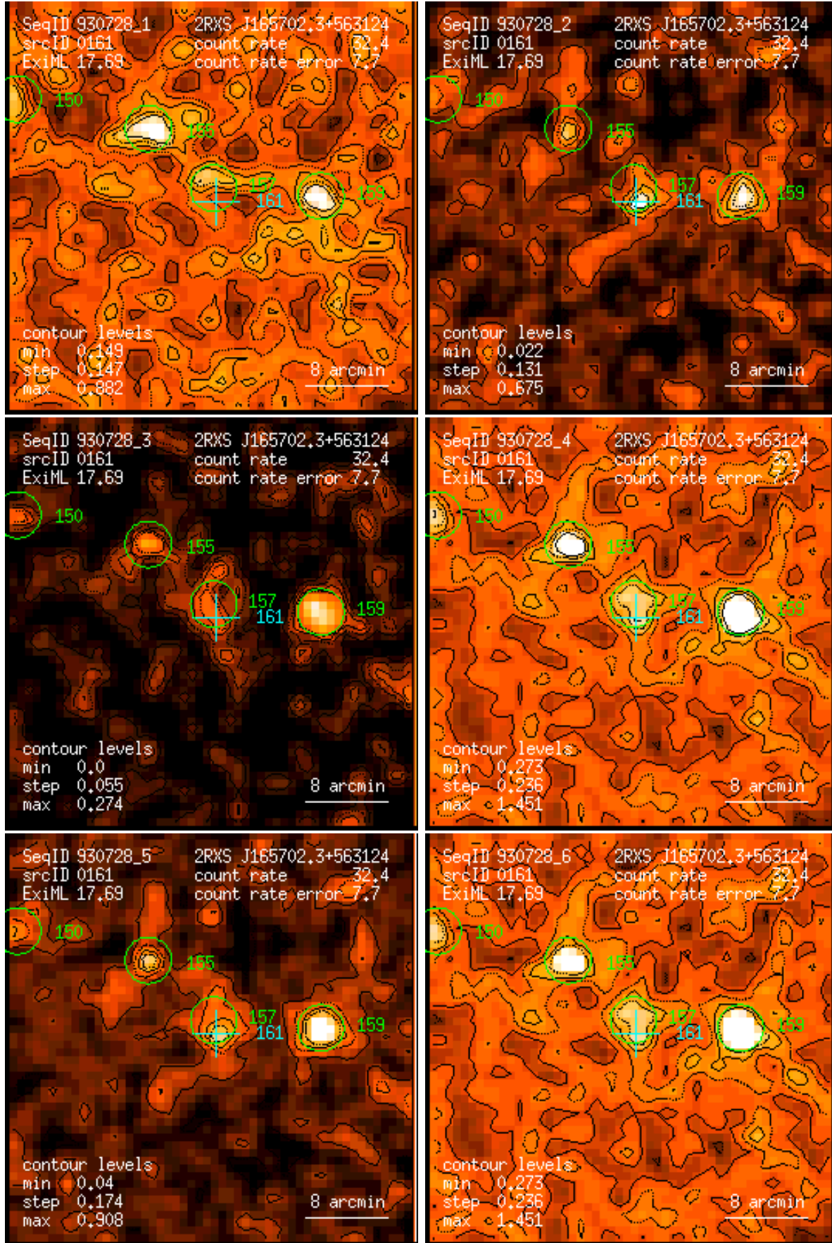
Figure 161: RASS 930728: detection 0161: band rate images, Gaussian filter: (1) PSPC channels 11 – 41, (2) 52 – 90, (3) 91 – 201, (4) 11 – 235, (5) 52 – 201, (6) 11 – 201. Broad band rates in counts/ks. Band rate contour levels in counts/ks/arcmin 2 .
