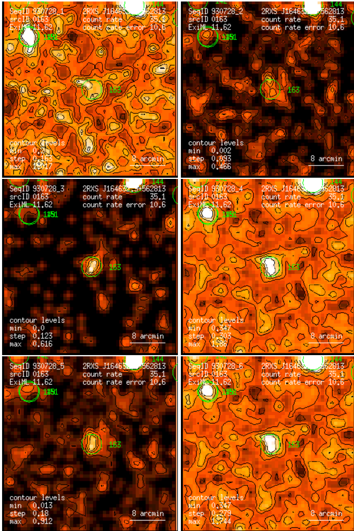
Figure 163: RASS 930728: detection 0163: band rate images, Gaussian filter: (1) PSPC channels 11 – 41, (2) 52 – 90, (3) 91 – 201, (4) 11 – 235, (5) 52 – 201, (6) 11 – 201. Broad band rates in counts/ks. Band rate contour levels in counts/ks/arcmin 2 .
