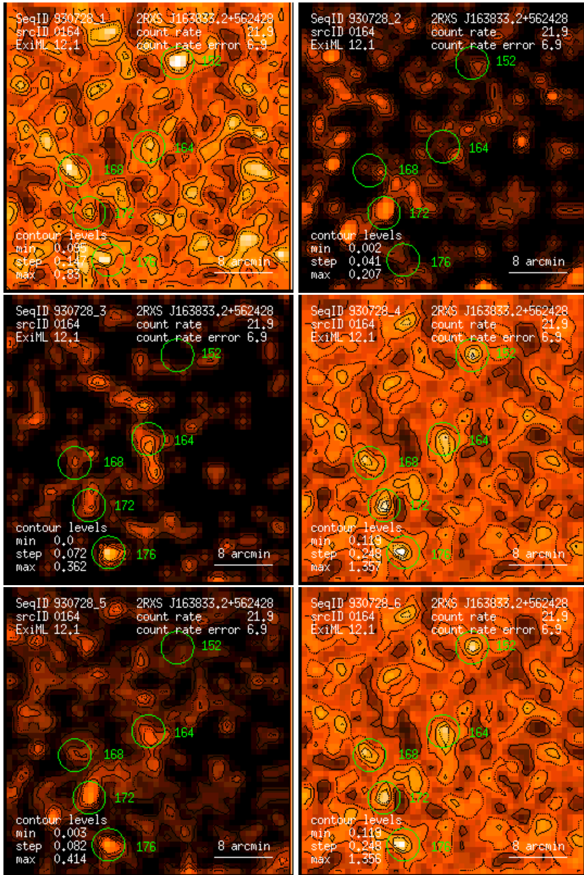
Figure 164: RASS 930728: detection 0164: band rate images, Gaussian filter: (1) PSPC channels 11 – 41, (2) 52 – 90, (3) 91 – 201, (4) 11 – 235, (5) 52 – 201, (6) 11 – 201. Broad band rates in counts/ks. Band rate contour levels in counts/ks/arcmin 2 .
