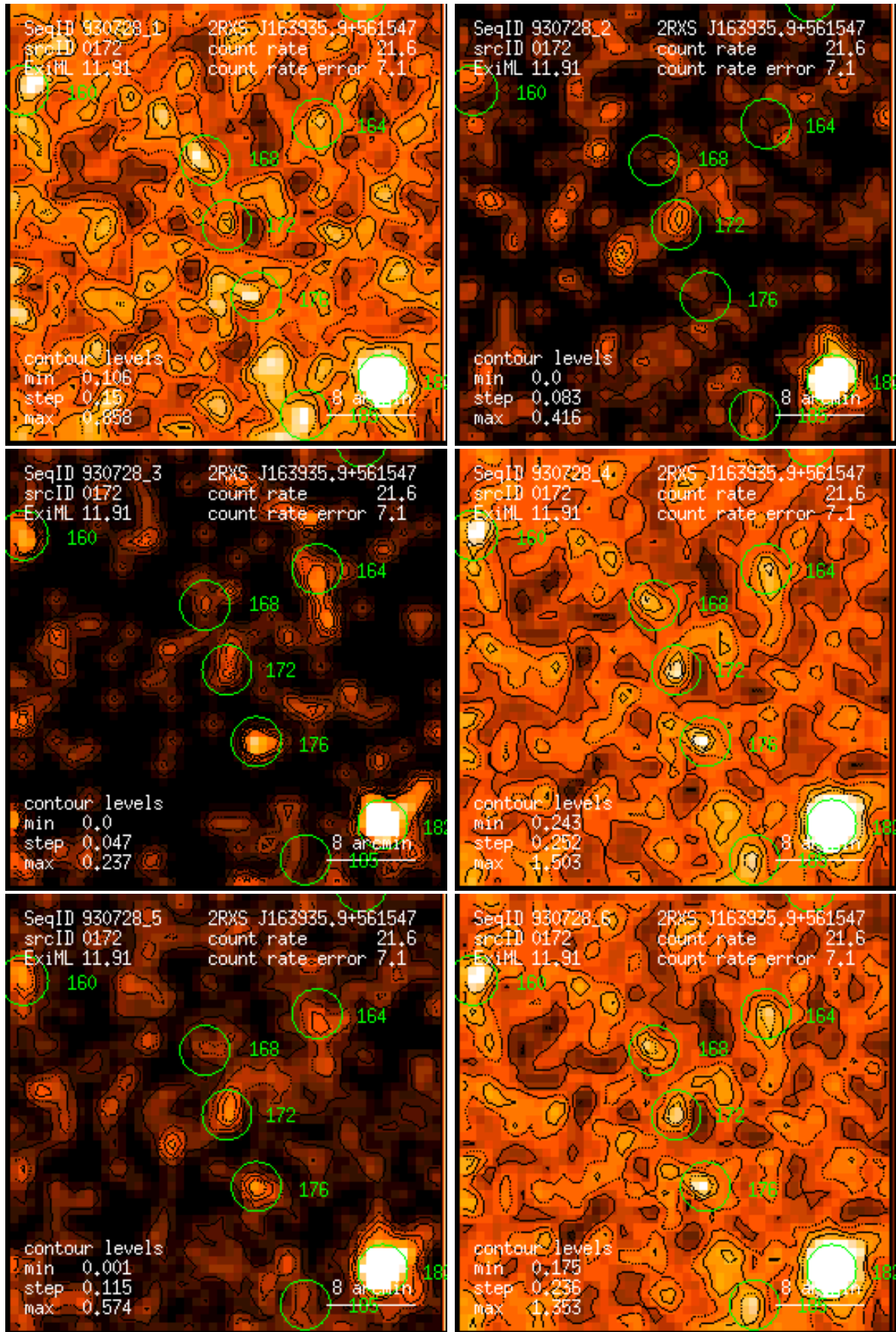
Figure 172: RASS 930728: detection 0172: band rate images, Gaussian filter: (1) PSPC channels 11 – 41, (2) 52 – 90, (3) 91 – 201, (4) 11 – 235, (5) 52 – 201, (6) 11 – 201. Broad band rates in counts/ks. Band rate contour levels in counts/ks/arcmin 2 .
