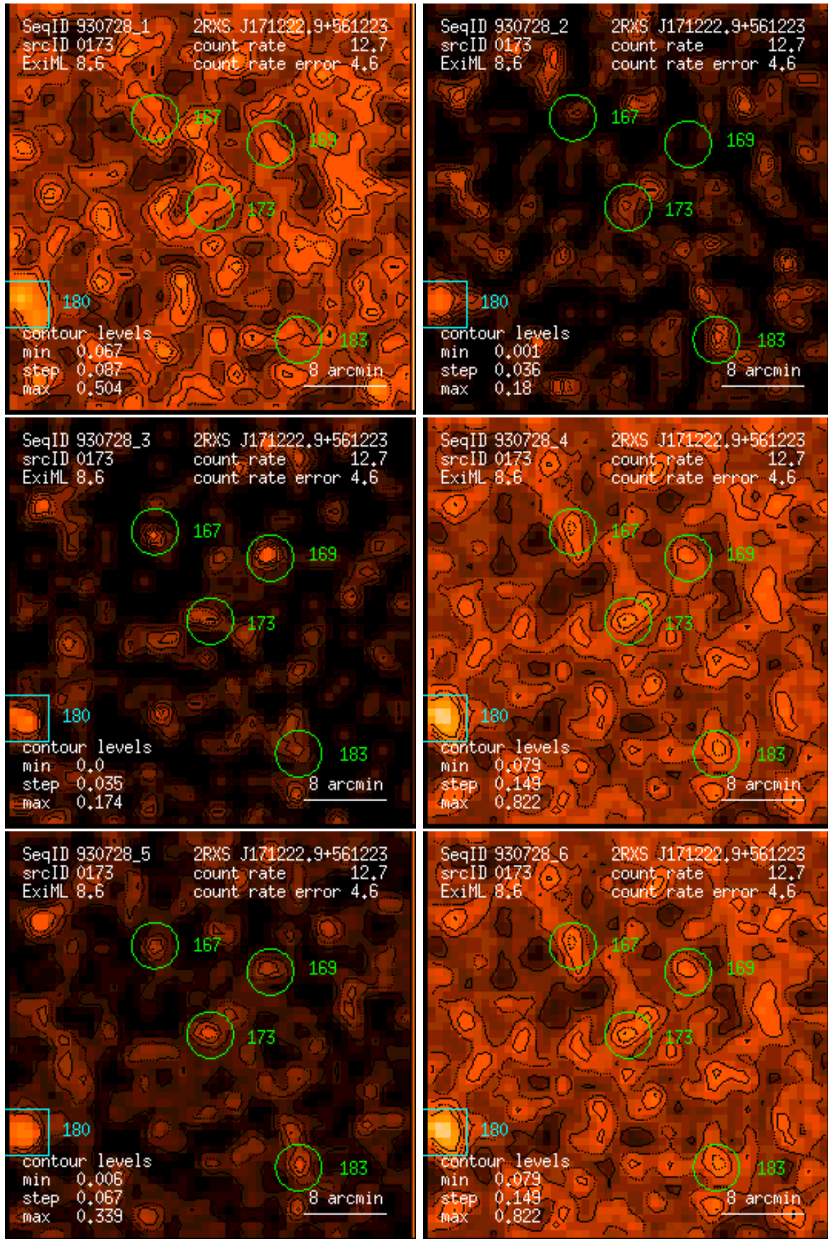
Figure 173: RASS 930728: detection 0173: band rate images, Gaussian filter: (1) PSPC channels 11 – 41, (2) 52 – 90, (3) 91 – 201, (4) 11 – 235, (5) 52 – 201, (6) 11 – 201. Broad band rates in counts/ks. Band rate contour levels in counts/ks/arcmin 2 .
