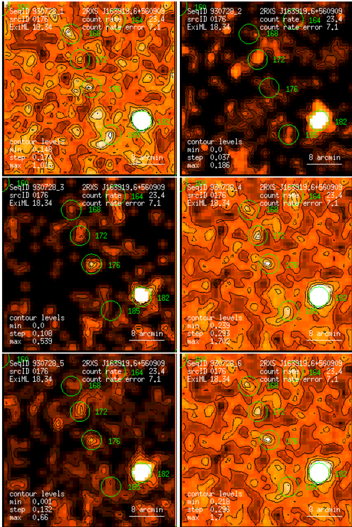
Figure 176: RASS 930728: detection 0176: band rate images, Gaussian filter: (1) PSPC channels 11 – 41, (2) 52 – 90, (3) 91 – 201, (4) 11 – 235, (5) 52 – 201, (6) 11 – 201. Broad band rates in counts/ks. Band rate contour levels in counts/ks/arcmin 2 .
