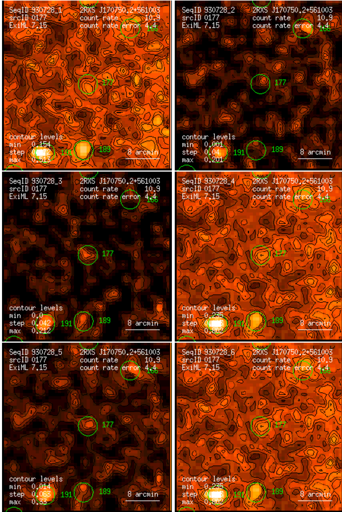
Figure 177: RASS 930728: detection 0177: band rate images, Gaussian filter: (1) PSPC channels 11 – 41, (2) 52 – 90, (3) 91 – 201, (4) 11 – 235, (5) 52 – 201, (6) 11 – 201. Broad band rates in counts/ks. Band rate contour levels in counts/ks/arcmin 2 .
