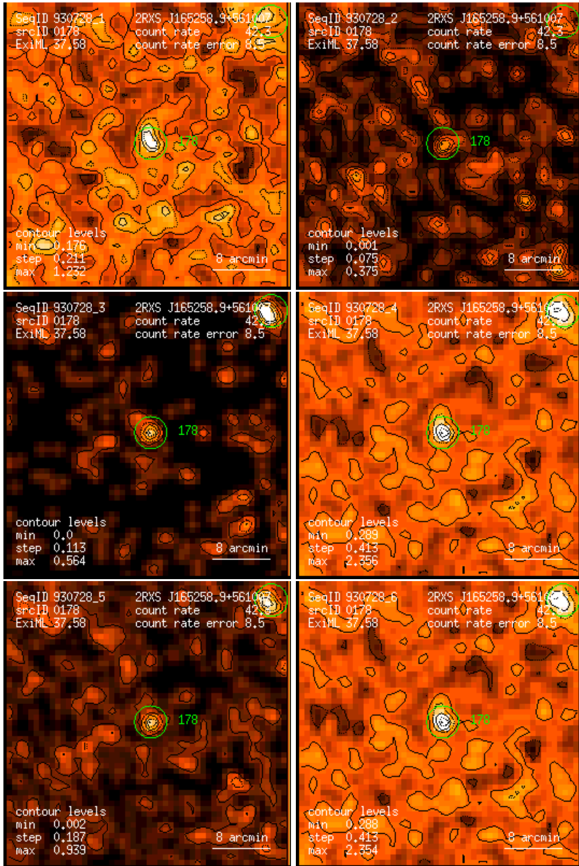
Figure 178: RASS 930728: detection 0178: band rate images, Gaussian filter: (1) PSPC channels 11 – 41, (2) 52 – 90, (3) 91 – 201, (4) 11 – 235, (5) 52 – 201, (6) 11 – 201. Broad band rates in counts/ks. Band rate contour levels in counts/ks/arcmin 2 .
