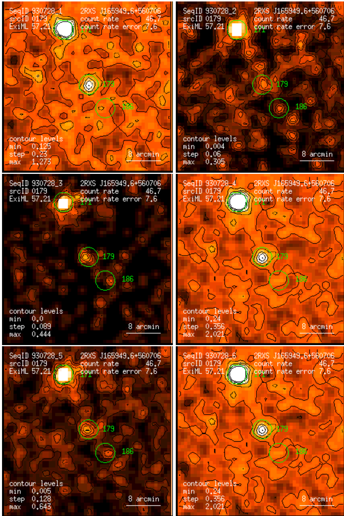
Figure 179: RASS 930728: detection 0179: band rate images, Gaussian filter: (1) PSPC channels 11 – 41, (2) 52 – 90, (3) 91 – 201, (4) 11 – 235, (5) 52 – 201, (6) 11 – 201. Broad band rates in counts/ks. Band rate contour levels in counts/ks/arcmin 2 .
