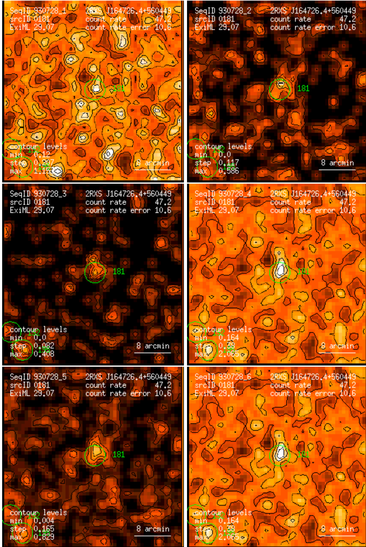
Figure 181: RASS 930728: detection 0181: band rate images, Gaussian filter: (1) PSPC channels 11 – 41, (2) 52 – 90, (3) 91 – 201, (4) 11 – 235, (5) 52 – 201, (6) 11 – 201. Broad band rates in counts/ks. Band rate contour levels in counts/ks/arcmin 2 .
