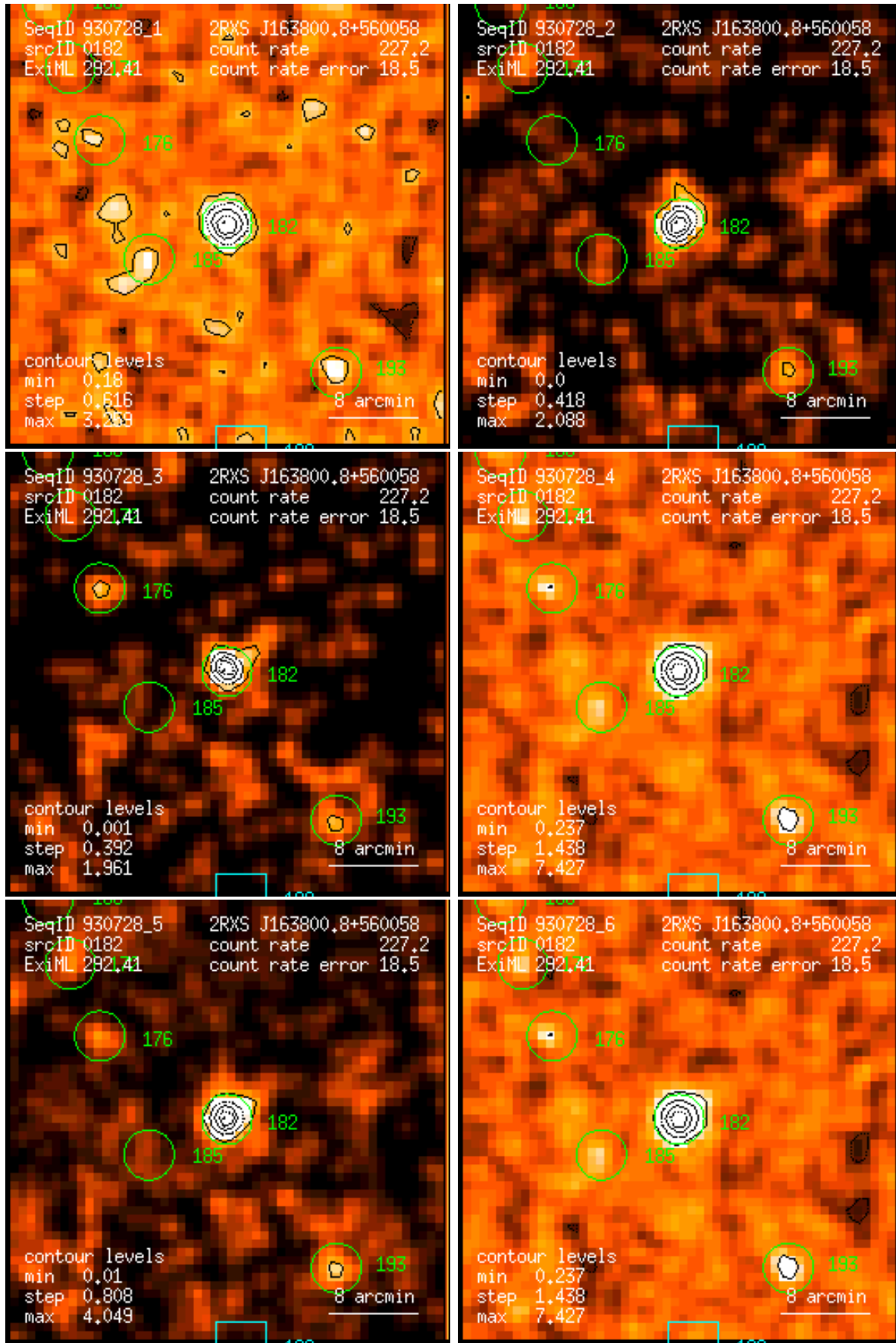
Figure 182: RASS 930728: detection 0182: band rate images, Gaussian filter: (1) PSPC channels 11 – 41, (2) 52 – 90, (3) 91 – 201, (4) 11 – 235, (5) 52 – 201, (6) 11 – 201. Broad band rates in counts/ks. Band rate contour levels in counts/ks/arcmin 2 .
