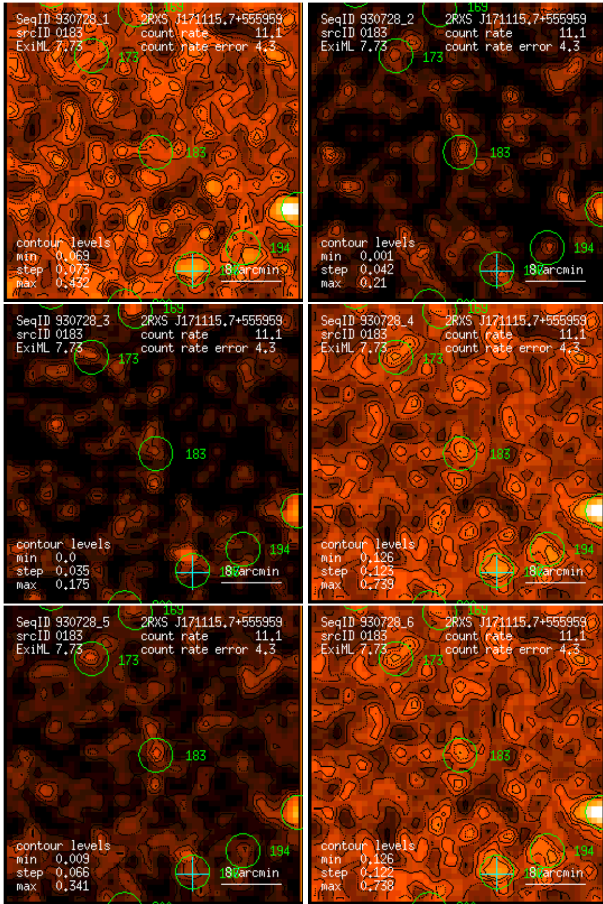
Figure 183: RASS 930728: detection 0183: band rate images, Gaussian filter: (1) PSPC channels 11 – 41, (2) 52 – 90, (3) 91 – 201, (4) 11 – 235, (5) 52 – 201, (6) 11 – 201. Broad band rates in counts/ks. Band rate contour levels in counts/ks/arcmin 2 .
