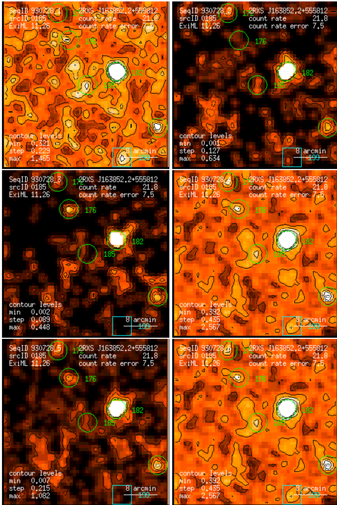
Figure 185: RASS 930728: detection 0185: band rate images, Gaussian filter: (1) PSPC channels 11 – 41, (2) 52 – 90, (3) 91 – 201, (4) 11 – 235, (5) 52 – 201, (6) 11 – 201. Broad band rates in counts/ks. Band rate contour levels in counts/ks/arcmin 2 .
