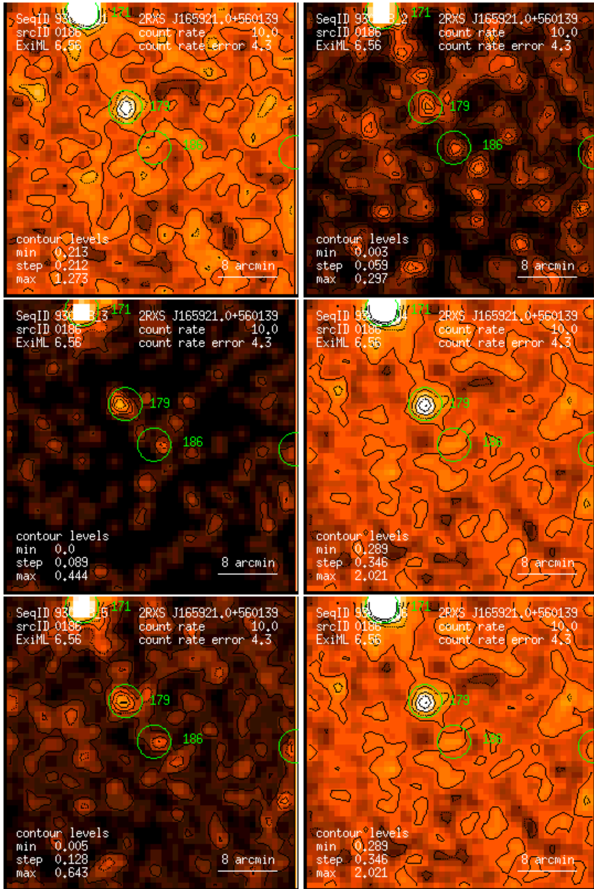
Figure 186: RASS 930728: detection 0186: band rate images, Gaussian filter: (1) PSPC channels 11 – 41, (2) 52 – 90, (3) 91 – 201, (4) 11 – 235, (5) 52 – 201, (6) 11 – 201. Broad band rates in counts/ks. Band rate contour levels in counts/ks/arcmin 2 .
