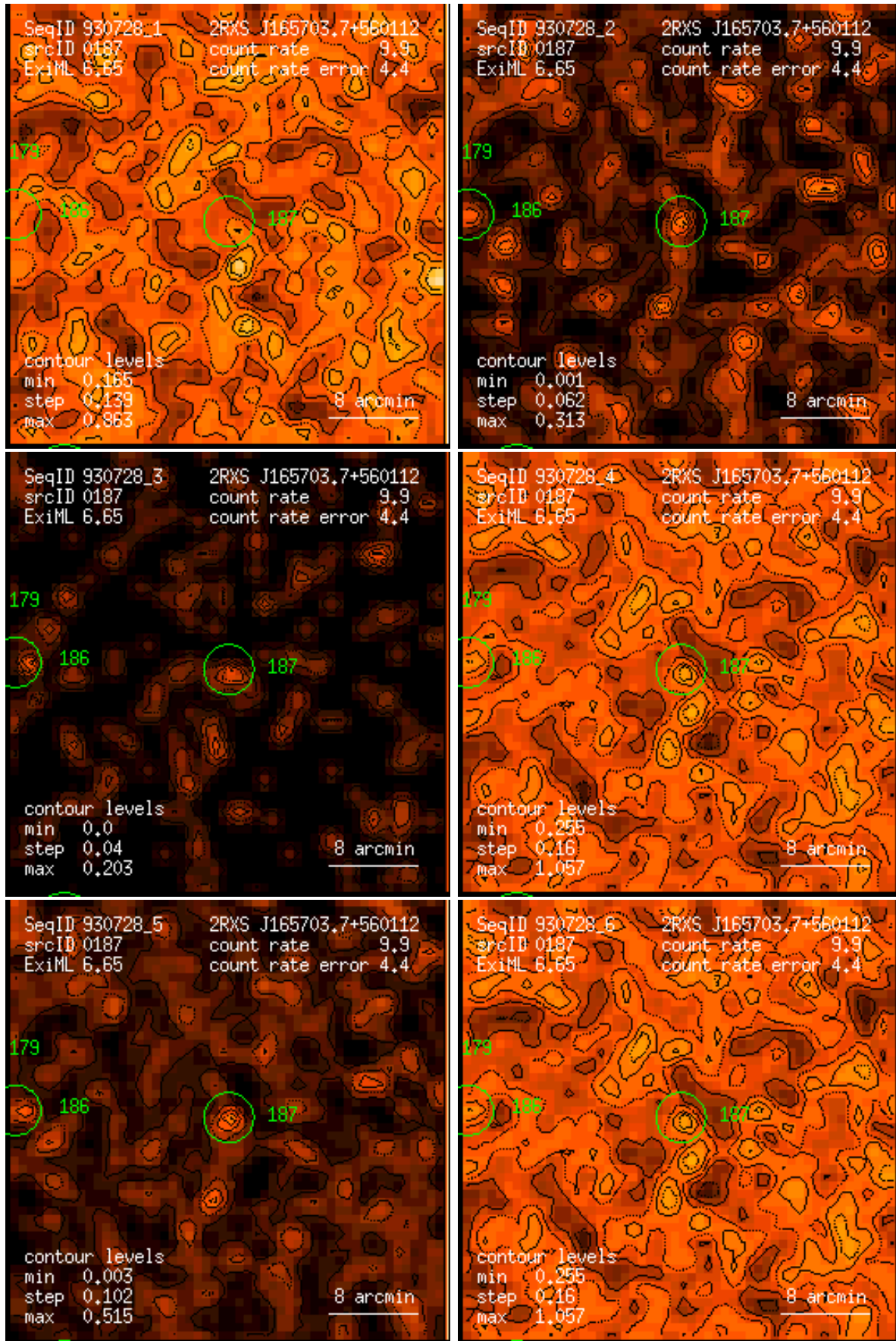
Figure 187: RASS 930728: detection 0187: band rate images, Gaussian filter: (1) PSPC channels 11 – 41, (2) 52 – 90, (3) 91 – 201, (4) 11 – 235, (5) 52 – 201, (6) 11 – 201. Broad band rates in counts/ks. Band rate contour levels in counts/ks/arcmin 2 .
