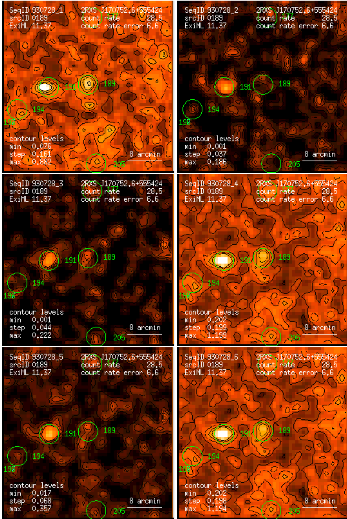
Figure 189: RASS 930728: detection 0189: band rate images, Gaussian filter: (1) PSPC channels 11 – 41, (2) 52 – 90, (3) 91 – 201, (4) 11 – 235, (5) 52 – 201, (6) 11 – 201. Broad band rates in counts/ks. Band rate contour levels in counts/ks/arcmin 2 .
