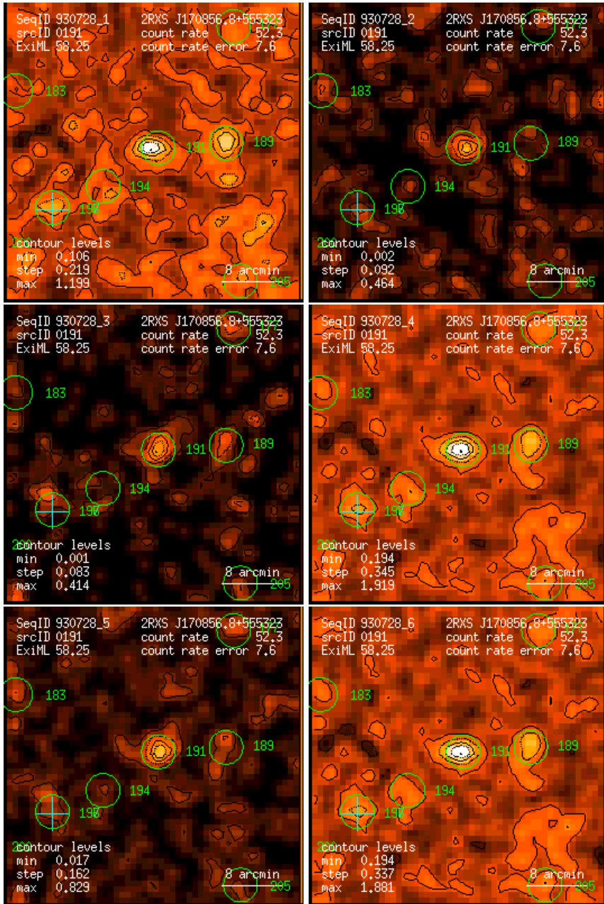
Figure 191: RASS 930728: detection 0191: band rate images, Gaussian filter: (1) PSPC channels 11 – 41, (2) 52 – 90, (3) 91 – 201, (4) 11 – 235, (5) 52 – 201, (6) 11 – 201. Broad band rates in counts/ks. Band rate contour levels in counts/ks/arcmin 2 .
