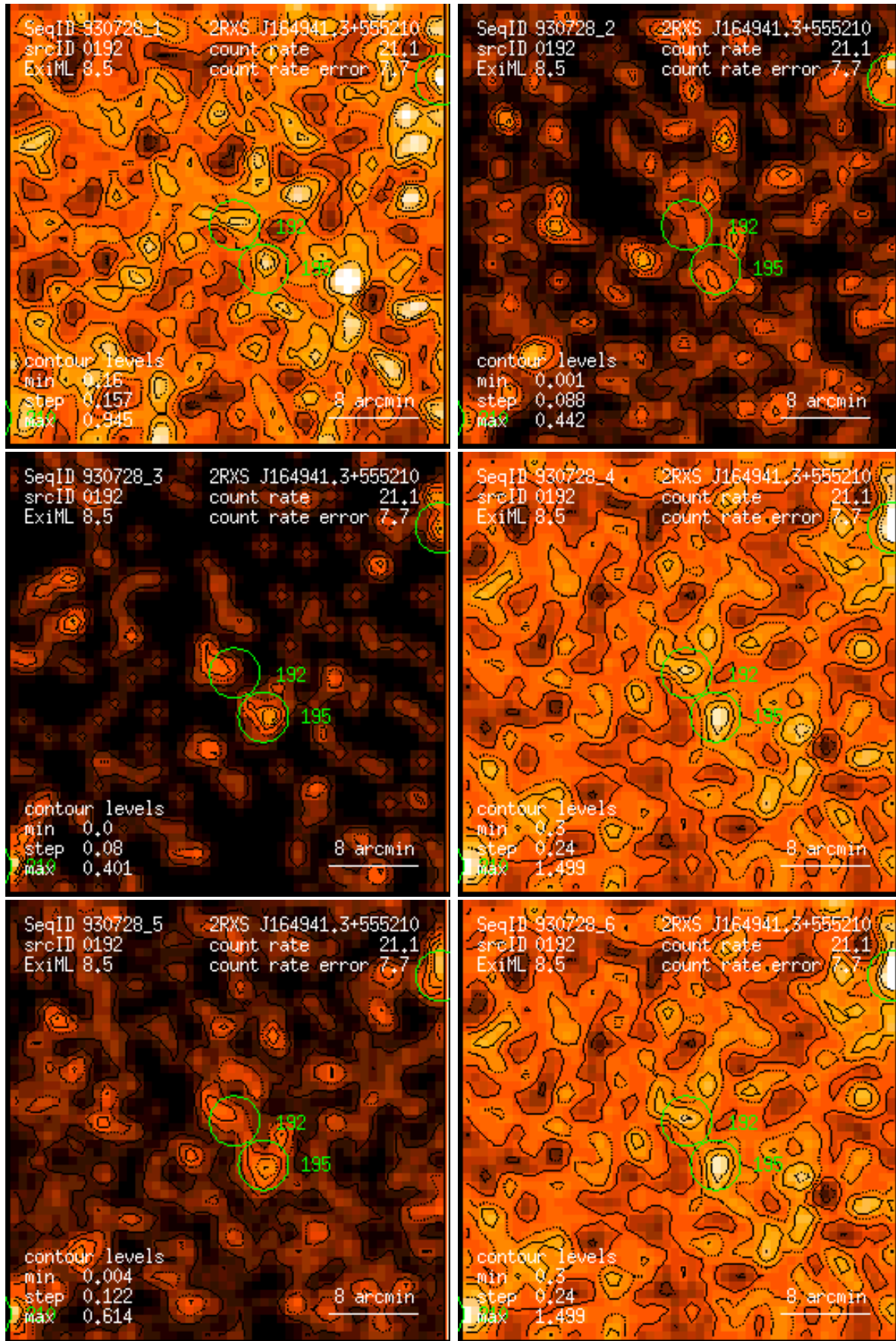
Figure 192: RASS 930728: detection 0192: band rate images, Gaussian filter: (1) PSPC channels 11 – 41, (2) 52 – 90, (3) 91 – 201, (4) 11 – 235, (5) 52 – 201, (6) 11 – 201. Broad band rates in counts/ks. Band rate contour levels in counts/ks/arcmin 2 .
