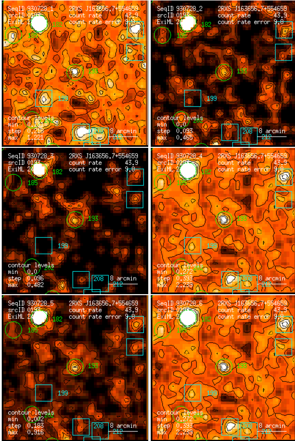
Figure 193: RASS 930728: detection 0193: band rate images, Gaussian filter: (1) PSPC channels 11 – 41, (2) 52 – 90, (3) 91 – 201, (4) 11 – 235, (5) 52 – 201, (6) 11 – 201. Broad band rates in counts/ks. Band rate contour levels in counts/ks/arcmin 2 .
