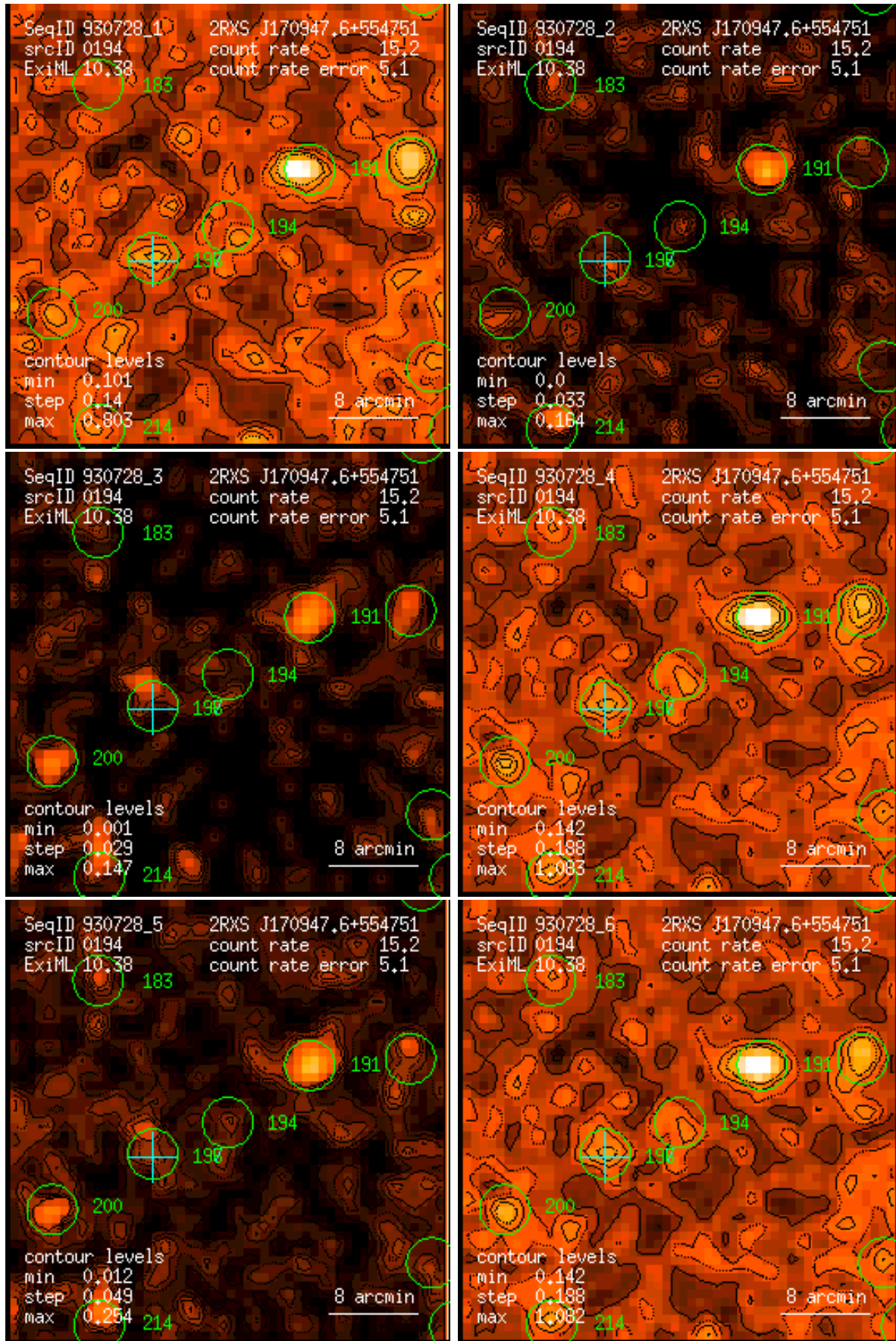
Figure 194: RASS 930728: detection 0194: band rate images, Gaussian filter: (1) PSPC channels 11 – 41, (2) 52 – 90, (3) 91 – 201, (4) 11 – 235, (5) 52 – 201, (6) 11 – 201. Broad band rates in counts/ks. Band rate contour levels in counts/ks/arcmin 2 .
