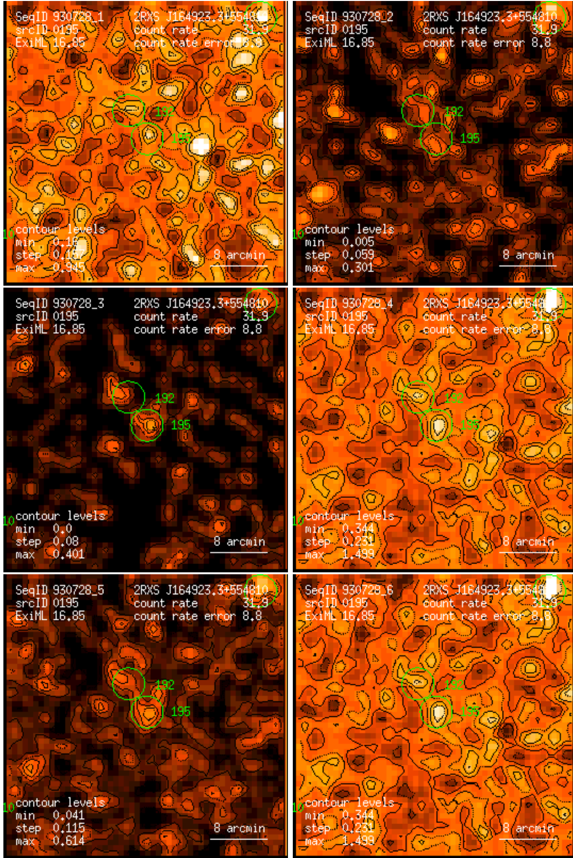
Figure 195: RASS 930728: detection 0195: band rate images, Gaussian filter: (1) PSPC channels 11 – 41, (2) 52 – 90, (3) 91 – 201, (4) 11 – 235, (5) 52 – 201, (6) 11 – 201. Broad band rates in counts/ks. Band rate contour levels in counts/ks/arcmin 2 .
