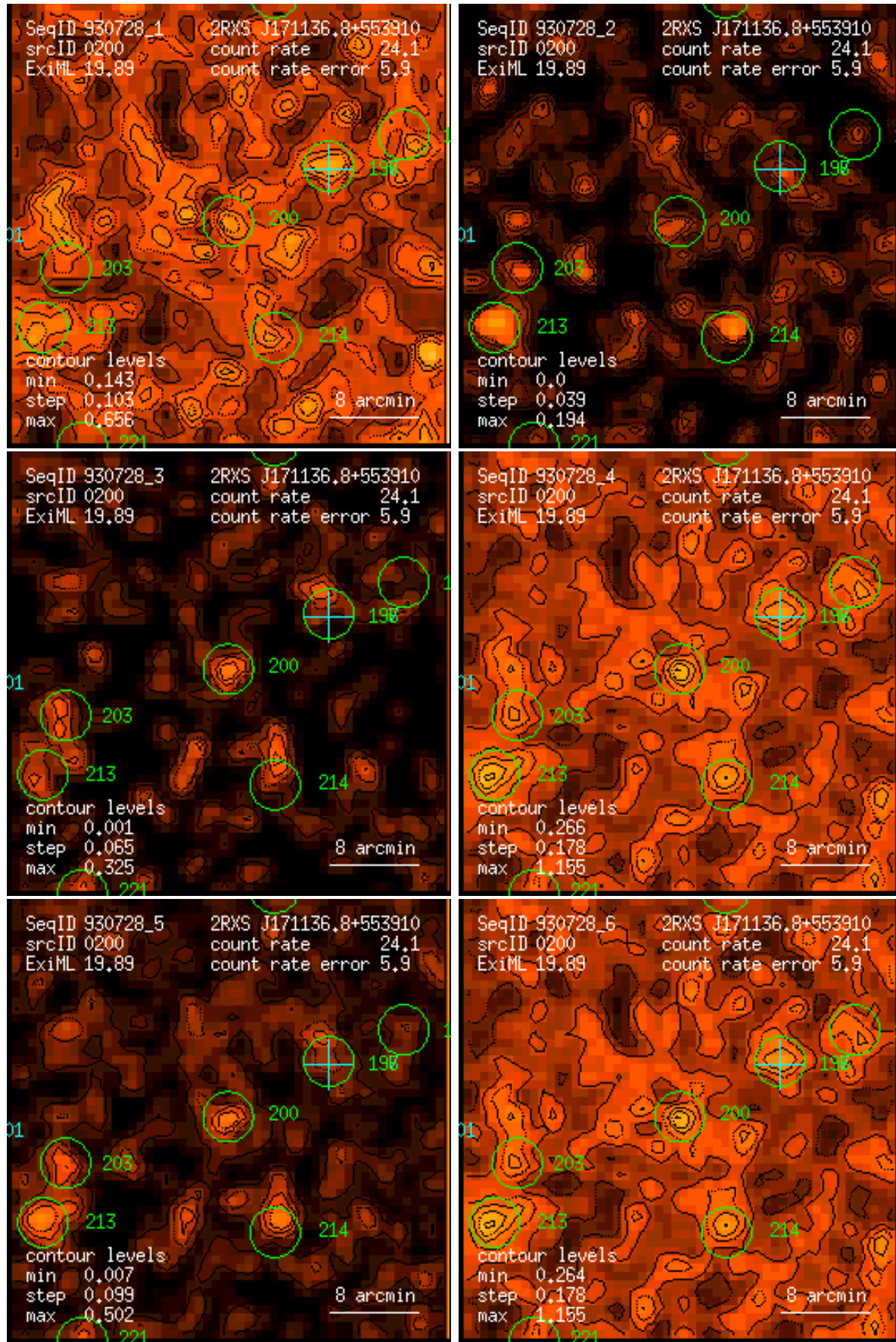
Figure 200: RASS 930728: detection 0200: band rate images, Gaussian filter: (1) PSPC channels 11 – 41, (2) 52 – 90, (3) 91 – 201, (4) 11 – 235, (5) 52 – 201, (6) 11 – 201. Broad band rates in counts/ks. Band rate contour levels in counts/ks/arcmin 2 .
