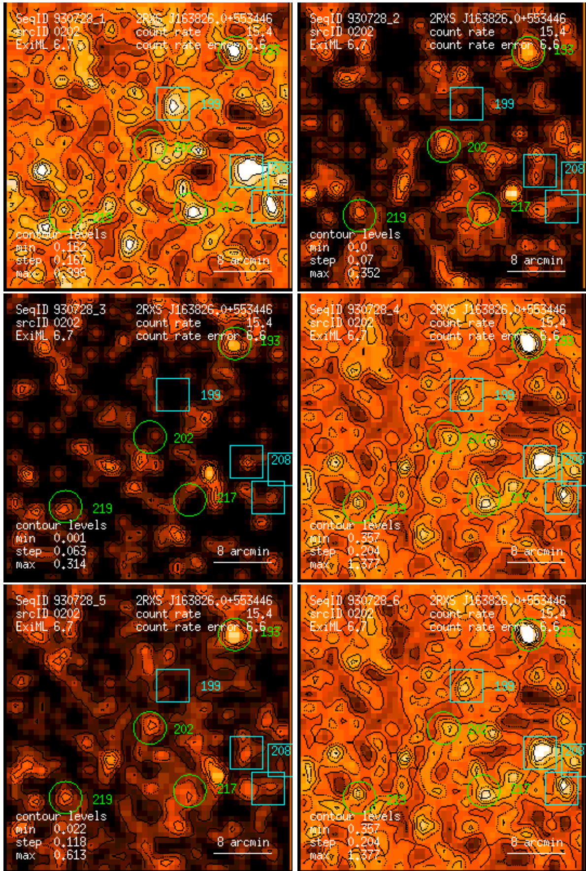
Figure 202: RASS 930728: detection 0202: band rate images, Gaussian filter: (1) PSPC channels 11 – 41, (2) 52 – 90, (3) 91 – 201, (4) 11 – 235, (5) 52 – 201, (6) 11 – 201. Broad band rates in counts/ks. Band rate contour levels in counts/ks/arcmin 2 .
