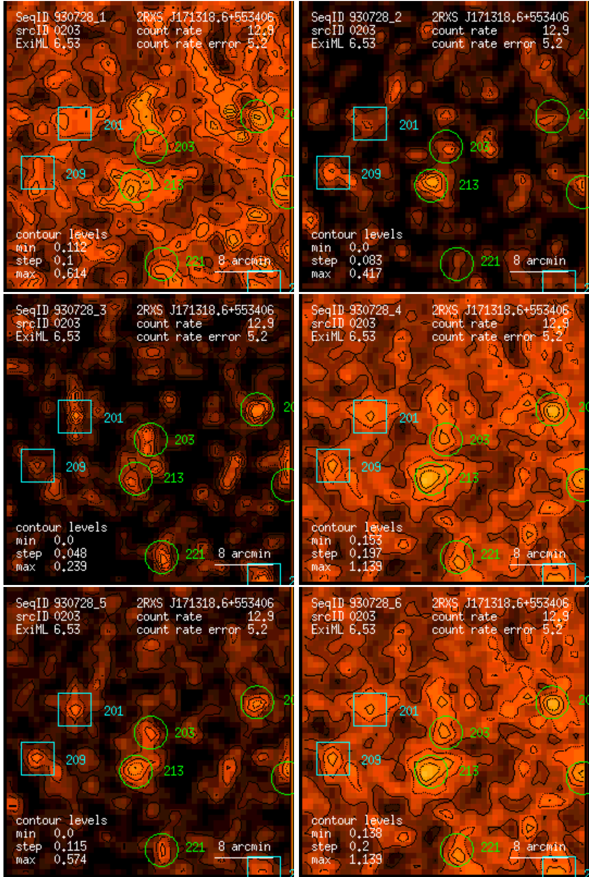
Figure 203: RASS 930728: detection 0203: band rate images, Gaussian filter: (1) PSPC channels 11 – 41, (2) 52 – 90, (3) 91 – 201, (4) 11 – 235, (5) 52 – 201, (6) 11 – 201. Broad band rates in counts/ks. Band rate contour levels in counts/ks/arcmin 2 .
