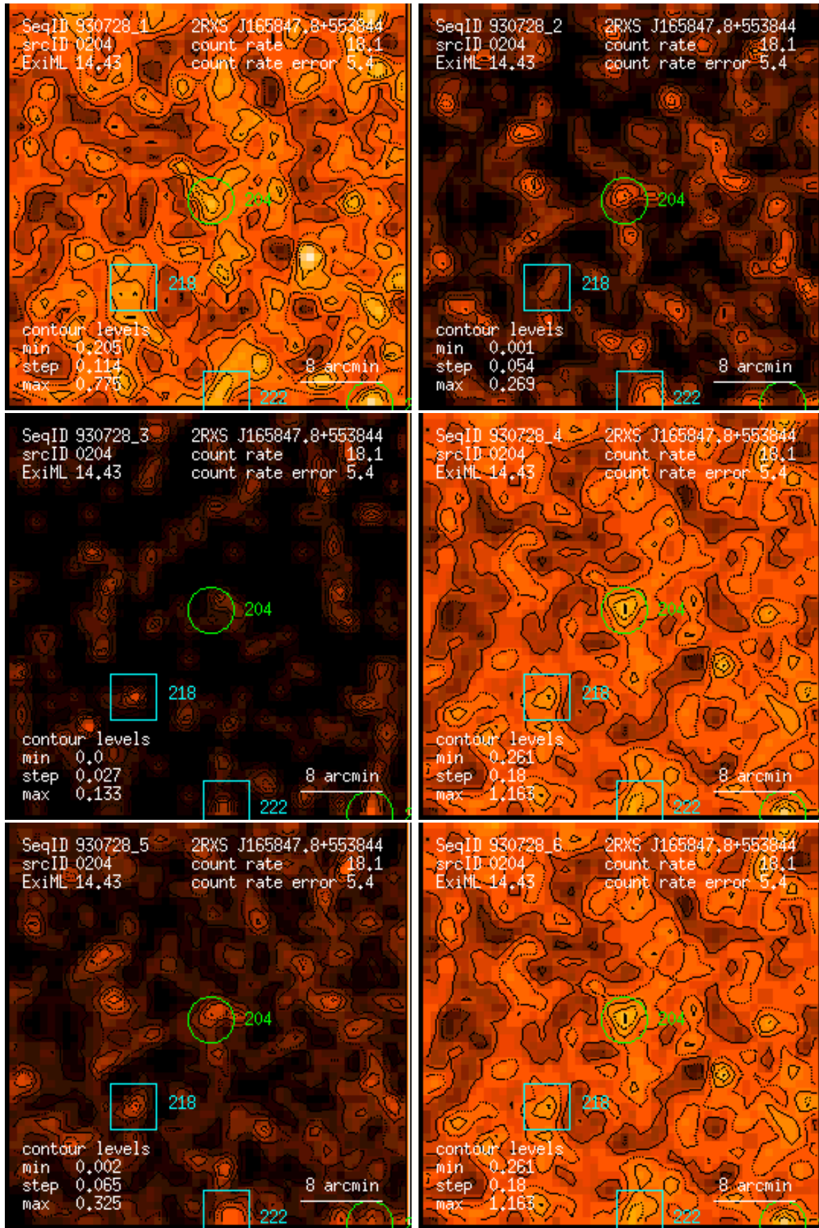
Figure 204: RASS 930728: detection 0204: band rate images, Gaussian filter: (1) PSPC channels 11 – 41, (2) 52 – 90, (3) 91 – 201, (4) 11 – 235, (5) 52 – 201, (6) 11 – 201. Broad band rates in counts/ks. Band rate contour levels in counts/ks/arcmin 2 .
