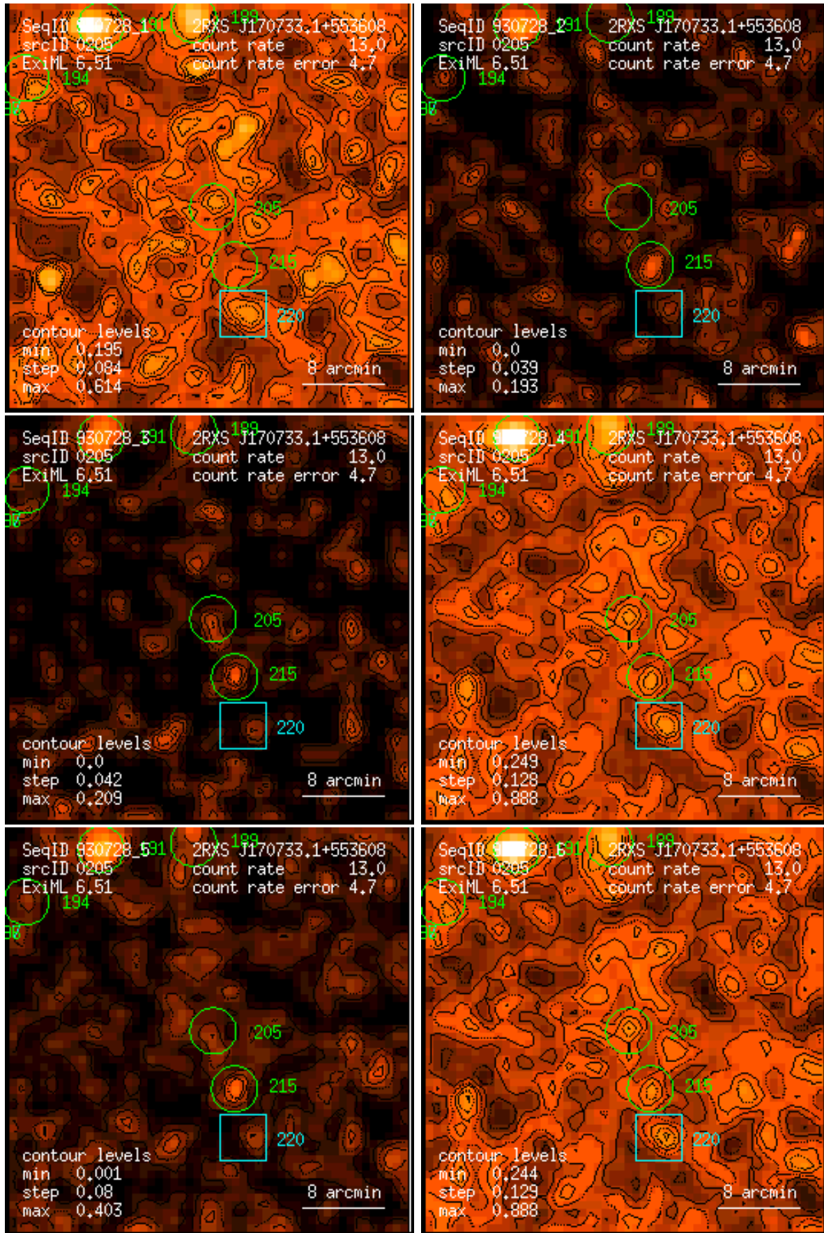
Figure 205: RASS 930728: detection 0205: band rate images, Gaussian filter: (1) PSPC channels 11 – 41, (2) 52 – 90, (3) 91 – 201, (4) 11 – 235, (5) 52 – 201, (6) 11 – 201. Broad band rates in counts/ks. Band rate contour levels in counts/ks/arcmin 2 .
