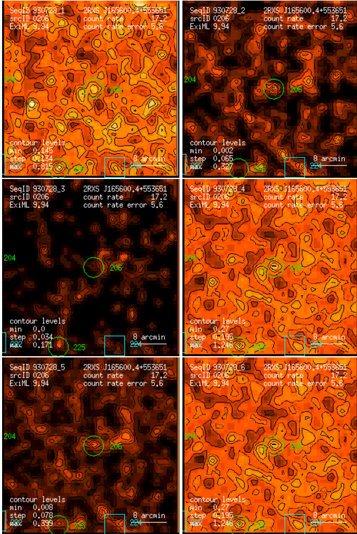
Figure 206: RASS 930728: detection 0206: band rate images, Gaussian filter: (1) PSPC channels 11 – 41, (2) 52 – 90, (3) 91 – 201, (4) 11 – 235, (5) 52 – 201, (6) 11 – 201. Broad band rates in counts/ks. Band rate contour levels in counts/ks/arcmin 2 .
