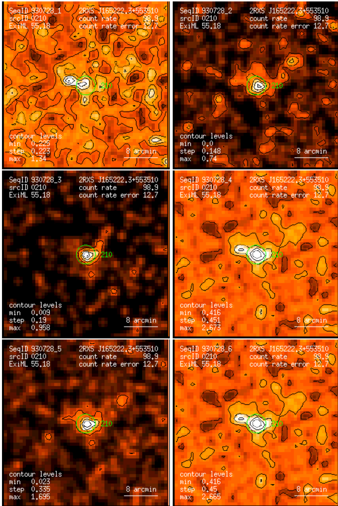
Figure 210: RASS 930728: detection 0210: band rate images, Gaussian filter: (1) PSPC channels 11 – 41, (2) 52 – 90, (3) 91 – 201, (4) 11 – 235, (5) 52 – 201, (6) 11 – 201. Broad band rates in counts/ks. Band rate contour levels in counts/ks/arcmin 2 .
