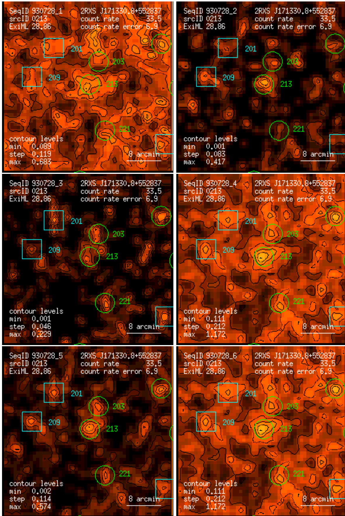
Figure 213: RASS 930728: detection 0213: band rate images, Gaussian filter: (1) PSPC channels 11 – 41, (2) 52 – 90, (3) 91 – 201, (4) 11 – 235, (5) 52 – 201, (6) 11 – 201. Broad band rates in counts/ks. Band rate contour levels in counts/ks/arcmin 2 .
