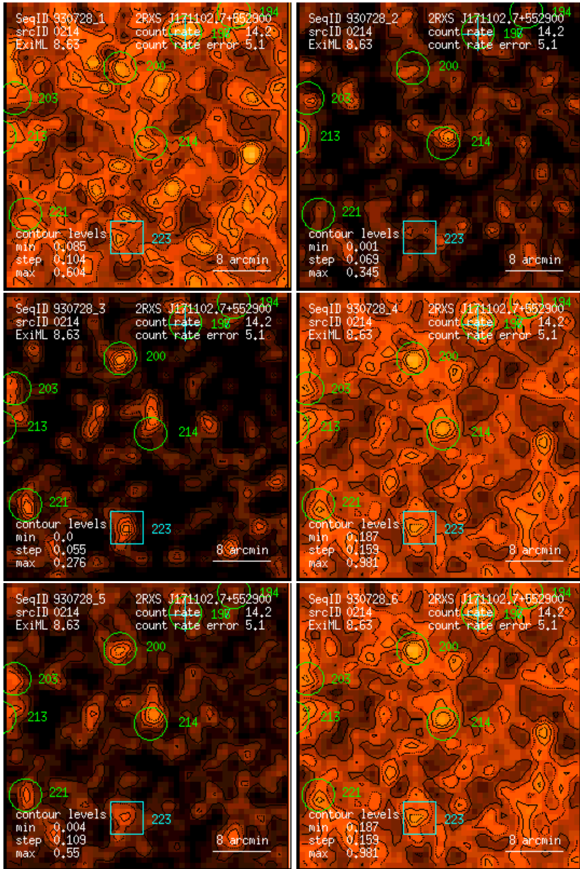
Figure 214: RASS 930728: detection 0214: band rate images, Gaussian filter: (1) PSPC channels 11 – 41, (2) 52 – 90, (3) 91 – 201, (4) 11 – 235, (5) 52 – 201, (6) 11 – 201. Broad band rates in counts/ks. Band rate contour levels in counts/ks/arcmin 2 .
