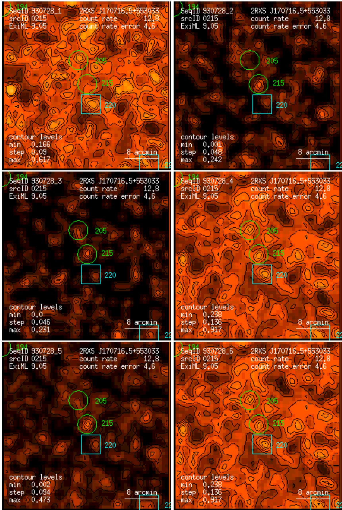
Figure 215: RASS 930728: detection 0215: band rate images, Gaussian filter: (1) PSPC channels 11 – 41, (2) 52 – 90, (3) 91 – 201, (4) 11 – 235, (5) 52 – 201, (6) 11 – 201. Broad band rates in counts/ks. Band rate contour levels in counts/ks/arcmin 2 .
