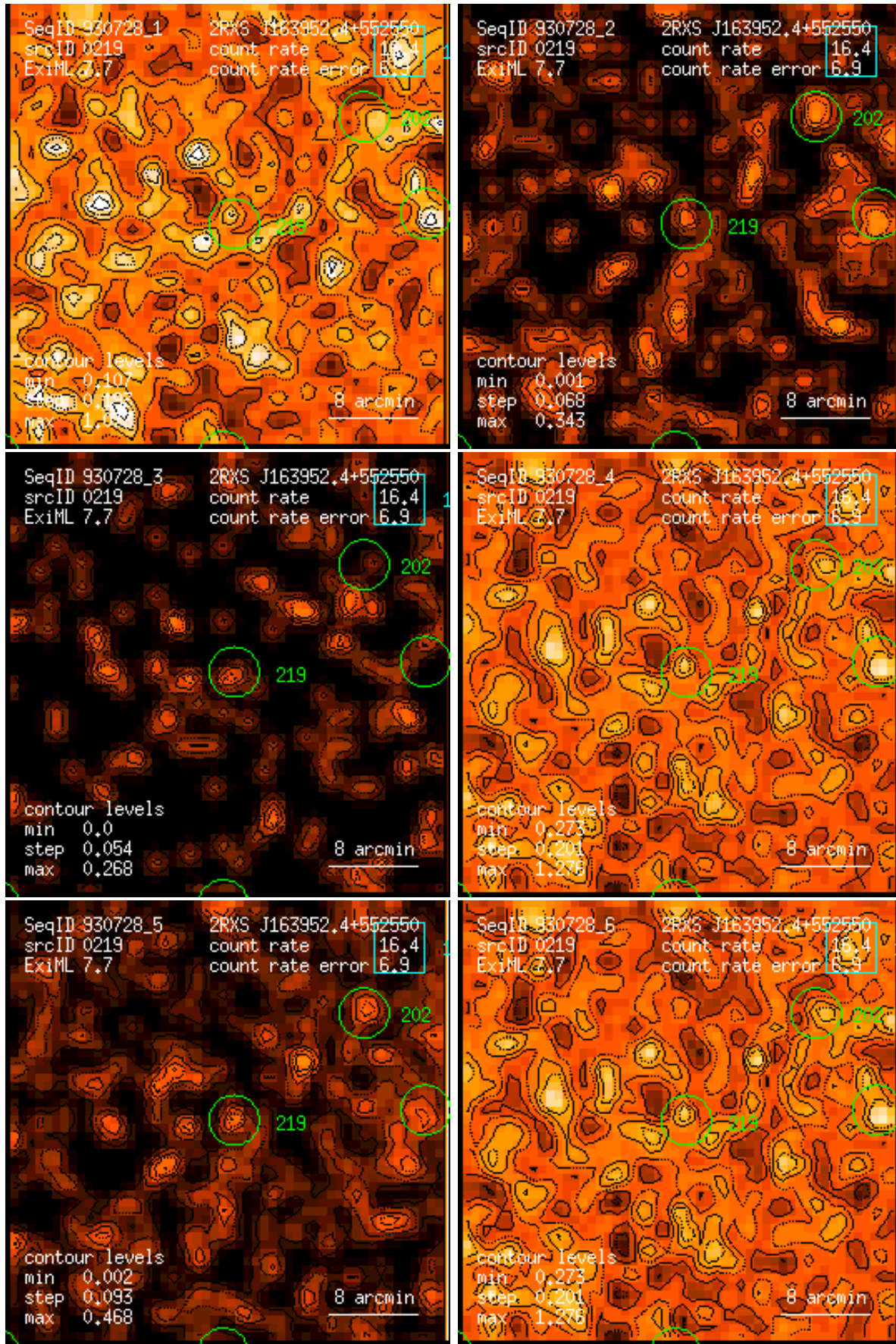
Figure 219: RASS 930728: detection 0219: band rate images, Gaussian filter: (1) PSPC channels 11 – 41, (2) 52 – 90, (3) 91 – 201, (4) 11 – 235, (5) 52 – 201, (6) 11 – 201. Broad band rates in counts/ks. Band rate contour levels in counts/ks/arcmin 2 .
